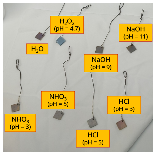
Figure 1: Samples after chemical treatments, before coating. From left to right, top to bottom the chemically treated samples are placed as water, \text{H}_2\text{O} , \text{H}_2\text{O}_2 , \text{NaOH} (pH 11), \text{NaOH} (pH 9), \text{NHO}_3 (pH 3), \text{NHO}_3 (pH 5), \text{HCl} (pH 3), \text{HCl} (pH 5), with the control sample not shown [9].
