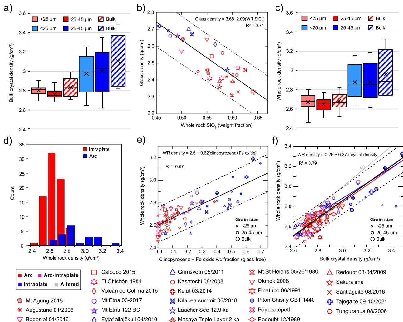
Figure 8. Density, chemistry, and size sensitivity. (a) Boxplots show bulk crystal density by size fraction for arc and intraplate samples. (b) The calculated glass density is sensitive to WR SiO 2 , as shown with a linear regression (solid black) and 95% confidence intervals for individual points (dashed lines). The regression has a poor fit for arc data alone. (c) Boxplots showing whole rock density with grain size; distributions for each tectonic setting are highlighted in (d). (e) Whole rock density is plotted against primary mineral fractions (e.g., glass- and secondary mineral-free) of clinopyroxene + Fe oxides. Bulk crystal and whole rock density if shown for all samples in (f). For panels (e) and (f), regressions are plotted for all non-altered samples (black, with 95% confidence limits for individual data points in dashed lines and equation given at top of plot). The 1:1 line and regression equation are shown. For panel (f) arc (red) and intraplate (blue) linear regressions are also shown.
