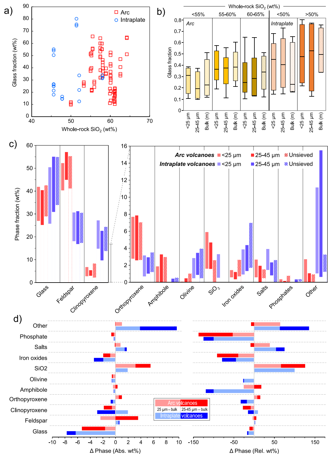
Figure 6. Average phase composition and sample standard error of the mean for arc and intraplate volcanic ash samples in the study. (a) Glass fraction is plotted against whole-rock SiO 2 for all samples, showing poor correlation and wide range. (b) Box plots showing glass content binned by whole-rock SiO 2 content and grain size. Arc samples are shown in yellow bars, intraplate samples in orange. (c) Sample standard deviation is shown as a bar for each phase for arc and intraplate ash samples. The y-axis scale is magnified for phases shown to the right of clinopyroxene to improve clarity of the minor phases. (d) Variations in phase abundance from the bulk for fine-sieved particles. Absolute variations (left) and relative variations (right) in weight fraction are plotted as stacked bars for each phase. Lighter colors represent the finest size range (< 25 μm) and darker colors the 25-45 μm range.
