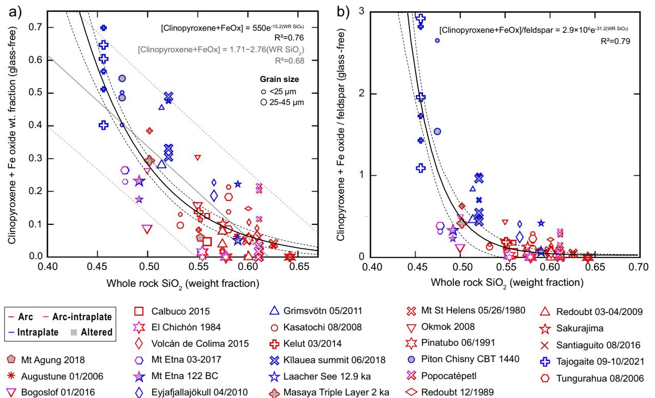
Figure 5. Scatter plots showing relationships between whole-rock SiO 2 and primary mineral phase fractions (labeled 'glass-free'). (a) Clinopyroxene + Fe oxides, normalized on a glass-free basis for < 25 and 25–45 \mu\text{m} fractions are fitted with an exponential regression (black line) and linear regression (grey line) to bulk silica with altered samples (symbols with grey fill) excluded. The grey dashed lines show the 95% confidence curves for individual data points; black dashed lines show 95% confidence for the exponential regression. (b) Identical to panel (a) , but with the y-axis divided by feldspar fraction and no linear regression shown. Dashed lines show 95% confidence limits for individual data points. Symbol size indicates sieve fraction (smallest = < 25 \mu\text{m} , largest = bulk (unsieved)). Equations for regressions with the coefficient of determination ( R^2 ) are shown.
