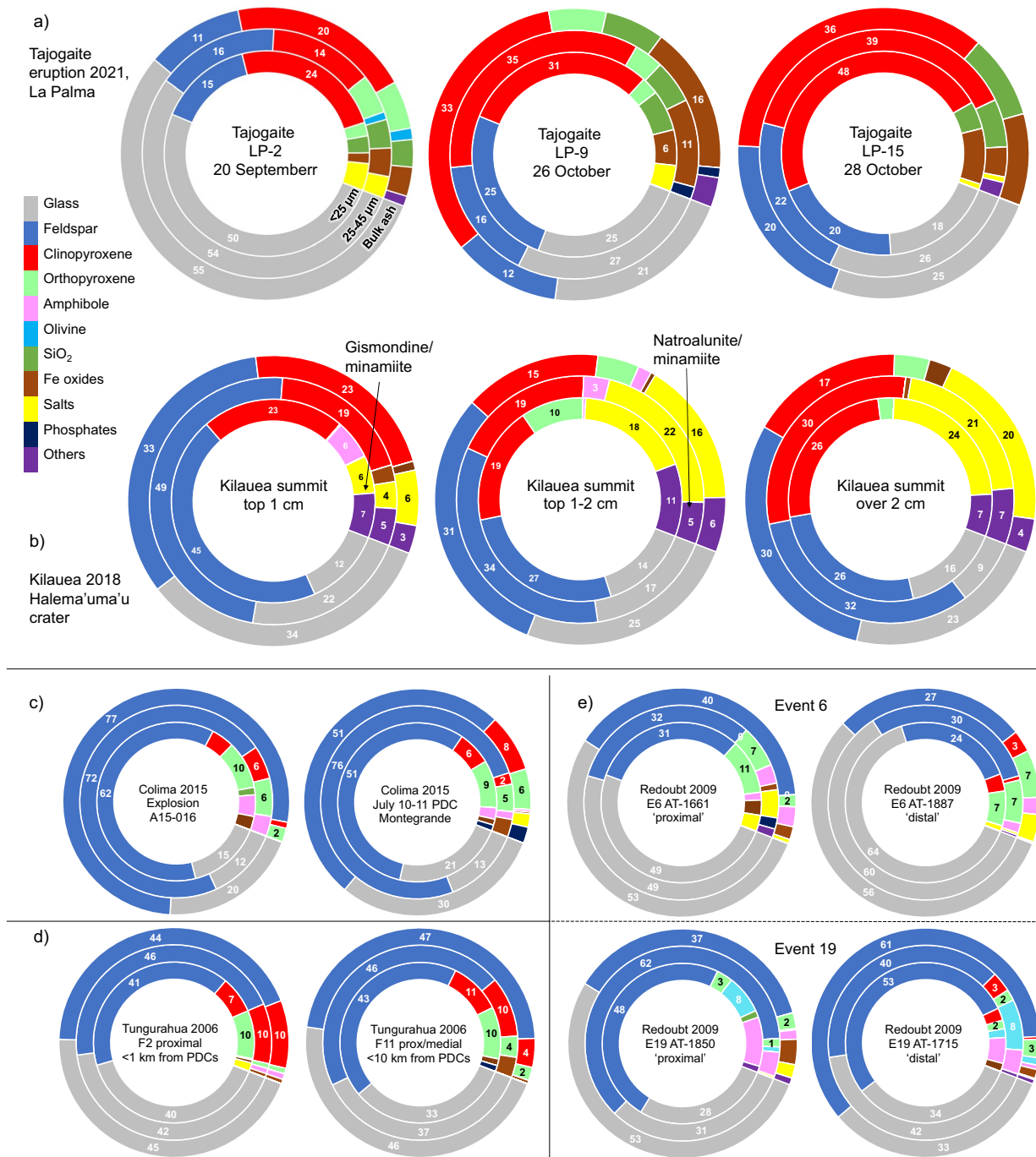
Figure 7. Variations in composition with distance and time. (a) Phase fractions for three airfall ash samples from the 2021 Tajogaite eruption on La Palma, Canary Islands, with size fractions nested in the donuts as labeled. Sample LP-2 was collected at the beginning of the eruption, while samples LP-9 and LP-15 were collected approximately one month later. (b) Kilauea ash sampled at varying depth from the summit caldera rim following the 2018 eruption. The identity of the most common phases grouped under 'Other' shown. (c) Volcán de Colima ash from an explosive event (left) and overbank PDC deposits (right), separated by approximately three months in 2015. (d) Two samples from the 2006 eruption of Tungurahua. Although the samples were collected at varying distances from the vent, the proximity to major PDCs appears to dominate the measured modal componentry and distance from PDC runout is given. (e) Two pairs of samples from the Redoubt 2009 eruption collected at relatively proximal and distal locations for two eruption episodes (Event 6 (E6) and Event 19 (E19)). An increase in glass fraction for the distal samples is clearly seen for Event 6 and for the sieved particles in Event 19.
