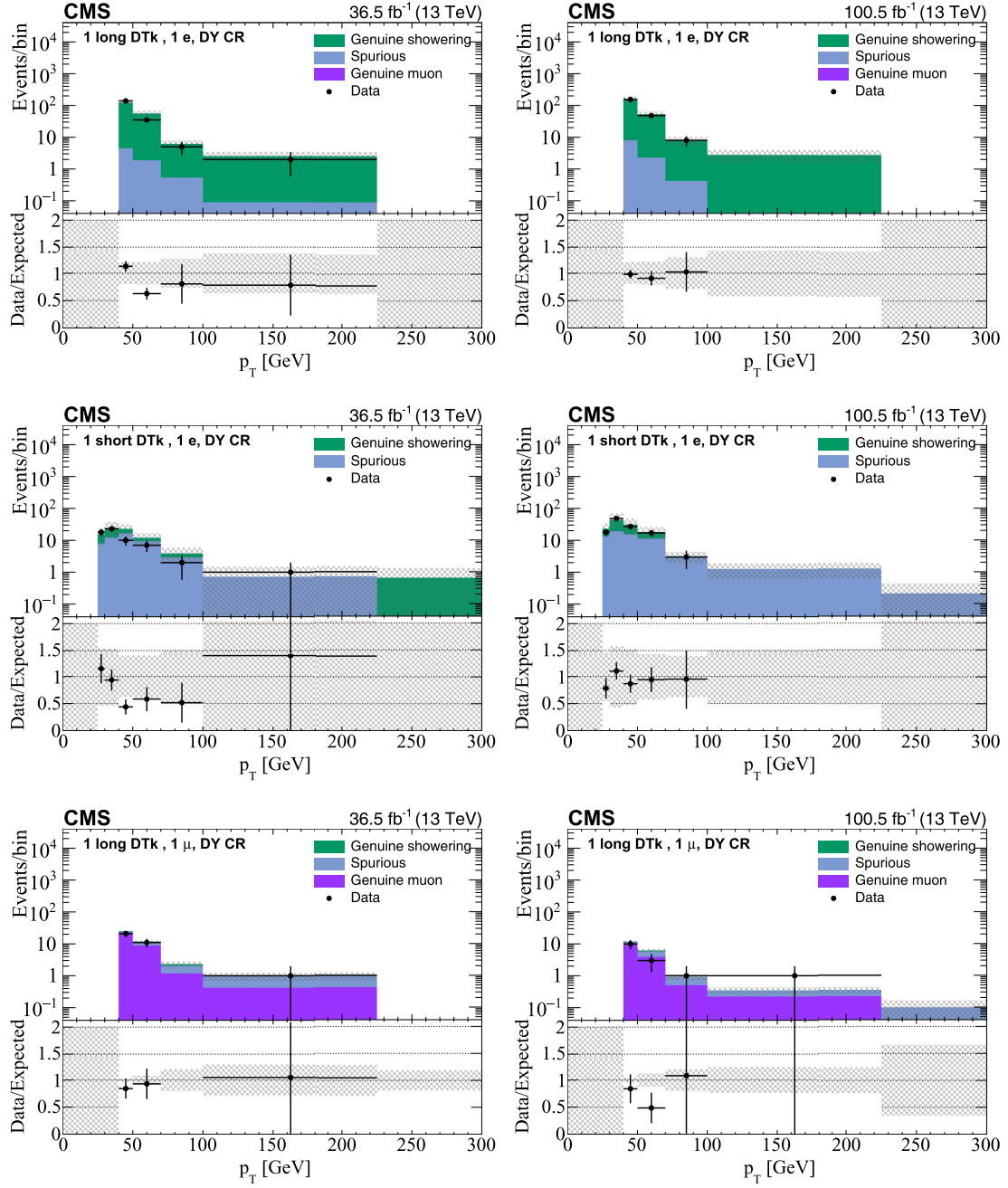
FIG. 3. Comparison of the p_T distributions of DTks in the \kappa^{\text{low}_{\text{high}}} DY measurement control region for the data and background prediction for long (upper) and short (middle) showering tracks and in the \kappa^{\mu_{\text{veto}}}_{\mu_{\text{match}}} DY measurement control region for long muon tracks (lower). The left (right) column corresponds to the phase-0 (phase-1) detector. The uncertainty bars on the ratios in the lower panels indicate the fractional Poisson uncertainties in the observed counts. The gray bands show the fractional Poisson uncertainties in the sideband region counts, added in quadrature with the systematic uncertainties. The leftmost (rightmost) bin includes underflow (overflow).
