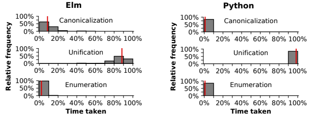
Fig. 12. COBBLER’s synthesis time broken down by time spent in canonicalization, unification, and enumeration. The data includes successful and unsuccessful runs, and vertical bars represent medians.
