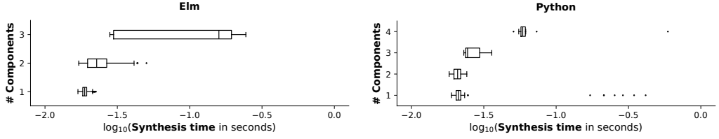
Fig. 6. COBBLER’s synthesis time on successful runs in the test set by language and number of components used. For all such runs, COBBLER provides a synthesis result in <1s. Whiskers are \pm 1.5 \times \text{IQR} .
