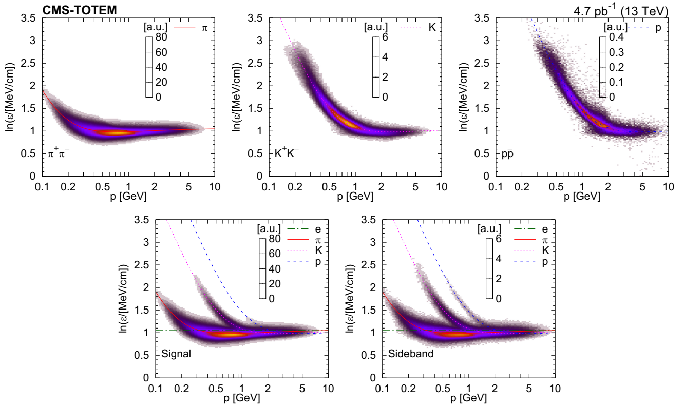
FIG. 6. Distribution of \ln \epsilon as a function of total momentum, for reconstructed charged particles in selected two-track events (identified \pi^+\pi^- , K^+K^- , p\bar{p} , signal, and sideband; Sec. V). The variable \epsilon is the most probable energy loss rate at a reference path length l_0 = 450 \mu\text{m} . The color scale is shown in arbitrary units and is linear. The curves show the expected \ln \epsilon for electrons, pions, kaons, and protons [Eq. (34.12) in Ref. [1]].
