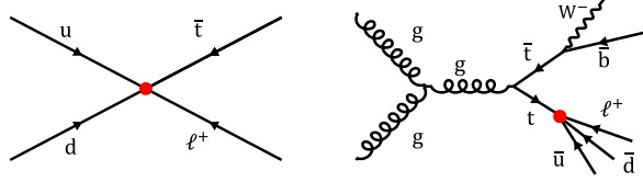
FIG. 1. Representative Feynman diagrams for single top quark production (left) and top quark decays (right) via BNV interactions. The red circles mark the BNV vertices.
