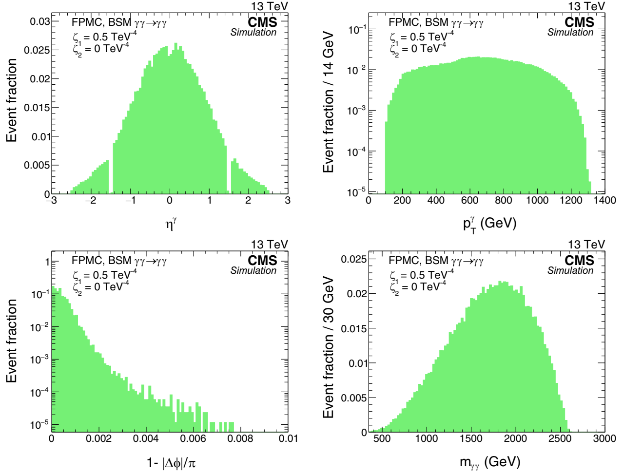
FIG. 3. Kinematic distributions of simulated aQGC \gamma\gamma \rightarrow \gamma\gamma events: Single-photon \eta (upper left) and p_T (upper right), and diphoton acoplanarity (lower left) and mass (lower right). The events are generated with FPMC, reconstructed accounting for the full CMS detector response, for aQGC parameters \zeta_1 = 0.5 \text{ TeV}^{-4} and \zeta_2 = 0 \text{ TeV}^{-4} . A preselection is applied to these events as described in Sec. V.
