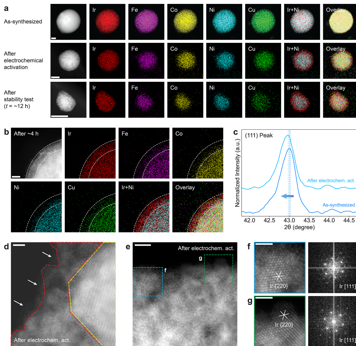
Figure 3. (a) STEM-EDX maps showing the elemental distribution of IrFeCoNiCu-HEA at different time points of the OER stability test (all scale bars: 20 nm). (b) STEM-EDX maps showing the Ir-rich shell layer near the surface of the nanoparticle, as highlighted by the dashed lines (scale bar: 10 nm). (c) Comparison of the (111) peaks from powder XRD measurement between as-synthesized and postelectrocatalysis samples showing a slight peak shift. (d) Near-surface structure of the nanoparticle showing the HEA core, polycrystalline alloy shell layer ( \sim 2\text{--}6 nm), and surface oxide (indicated by white arrows) after electrochemical activation. (e) HAADF-STEM image of IrFeCoNiCu-HEA near the surface showing the Ir-rich nanodomains (scale bar: 2 nm). (f, g) Ir domains populate the shell layer and surface of the nanoparticle, having different in-plane rotational angles (all scale bars: 1 nm).
