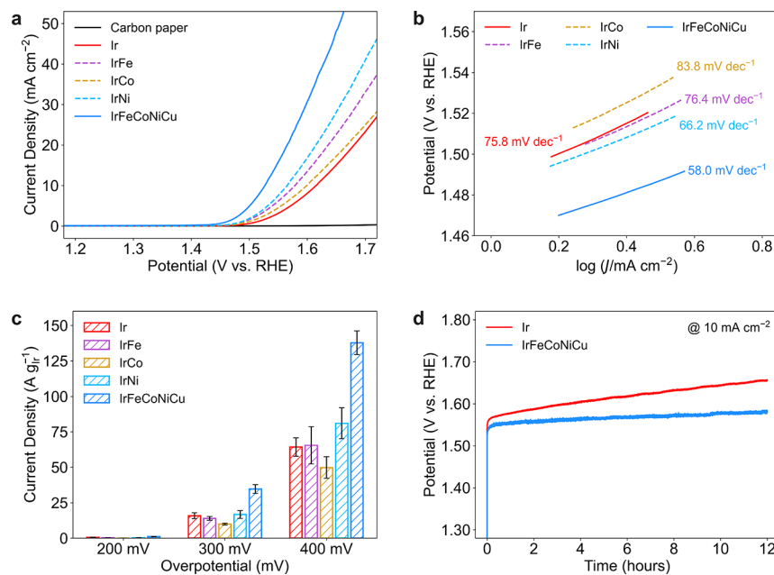
Figure 2. (a) OER polarization curves in 0.1 M HClO 4 electrolyte (scan rate, 5 mV s -1 ). (b) Corresponding Tafel slopes. (c) Ir-mass-based activity measured at different overpotentials. (d) Chronopotentiometry measurement at a constant current density of 10 mA cm -2 .
