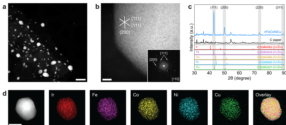
Figure 1. (a) Low-resolution HAADF-STEM image of IrFeCoNiCu-HEA dispersed on carbon paper substrate (scale bar: 500 nm). (b) High-resolution HAADF-STEM image (scale bar: 2 nm) and inset of the corresponding FFT showing a typical FCC structure. (c) XRD pattern of IrFeCoNiCu-HEA showing the single-phase FCC structure. (d) Homogeneous elemental distribution of IrFeCoNiCu-HEA shown by individual STEM-EDX maps and their overlay (scale bar: 50 nm).
