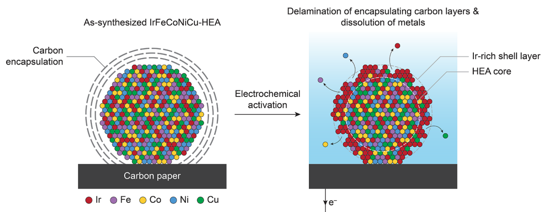
Figure 4. Illustration of the structural evolution of IrFeCoNiCu-HEA nanoparticle under acidic OER conditions. The electrocatalytic condition induces delamination of the encapsulating carbon layers and dissolution of mostly the 3d metals, leaving an Ir-rich shell layer on the surface of the nanoparticle.
