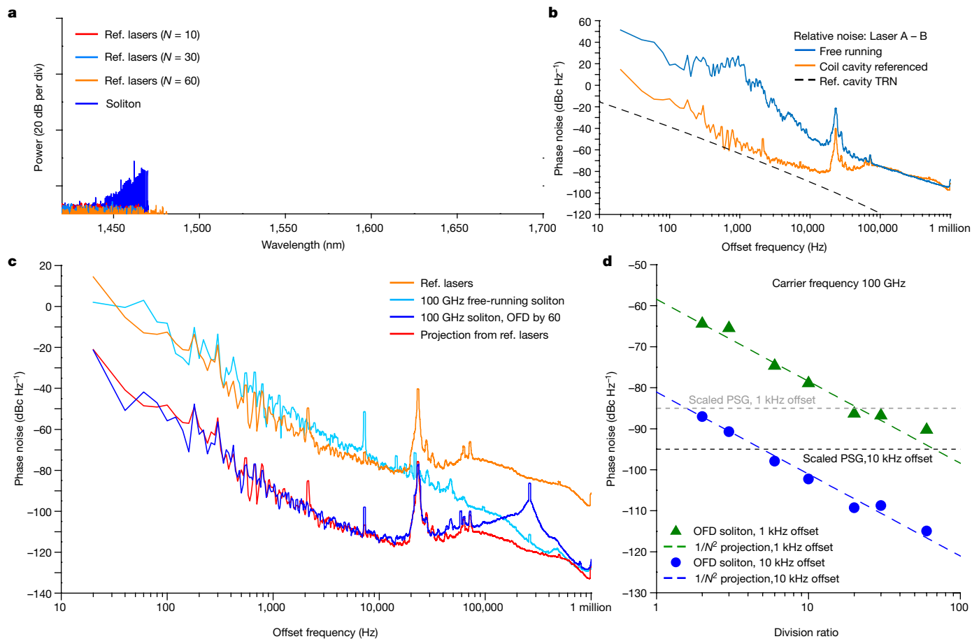
Fig. 3 | OFD characterization. a , Optical spectra of soliton microcombs (blue) and reference (Ref.) lasers corresponding to different division ratios. b , Phase noise of the frequency difference between the two reference lasers stabilized to coil cavity (orange) and the two lasers at free running (blue). The black dashed line shows the thermal refractive noise (TRN) limit of the reference cavity. c , Phase noise of reference lasers (orange), the repetition rate of
