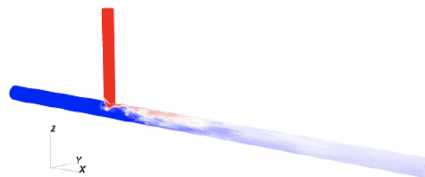
Figure 13. T-junction test case: instantaneous temperature field at Re = 10,000 for an investigation on thermal striping, which is critical in nuclear engineering [200].
