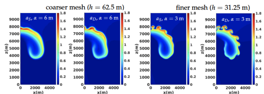
Figure 9. Rising thermal bubble: perturbation of potential temperature \theta' at t = 1020 s computed with the EFR and a_S and a_D with the coarser mesh (first two panels) and the finer mesh (last two panels).
