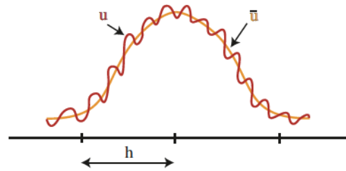
Figure 2. LES schematic showing the input flow variable, u , that cannot be represented on a given coarse mesh, and the filtered flow variable, \bar{u} , that can be accurately represented on the coarse mesh.
