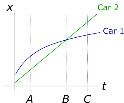
FIG. 8. The first of four isomorphic graph tasks adapted from Ref. [9]. The other three graph tasks are shown in detail in Appendix A. Note that this is the same task as that shown in Fig. 1.
