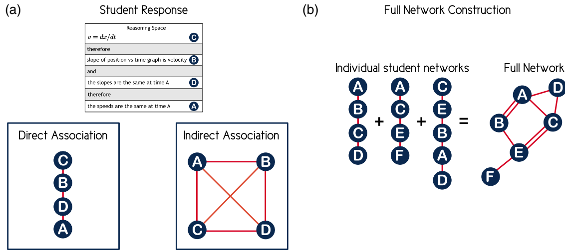
FIG. 2. (a) An example of two methods for constructing an individual-student network from an individual student's response. (b) An illustration of summing individual student networks to create a full network.
