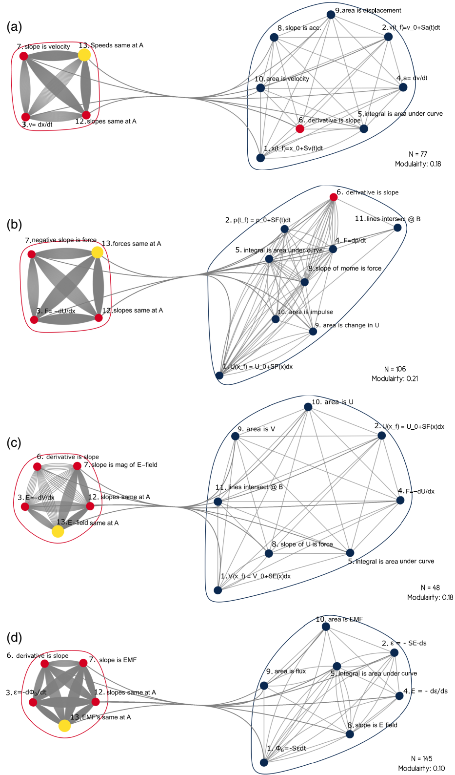
FIG. 10. Community structure detected in indirect association networks comprised of correct responses to the graph task as posed in the context of (a) kinematics, (b) potential energy, (c) electric potential, and (d) magnetic flux.
