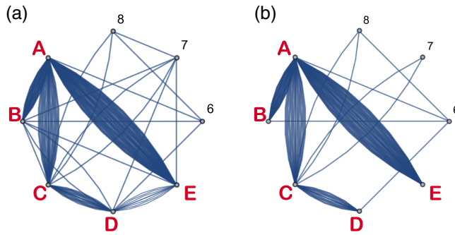
FIG. 11. Example network illustrating locally adaptive network sparsification [64]. (a) The base network. (b) The same network after sparsification at \alpha = 0.1 .
