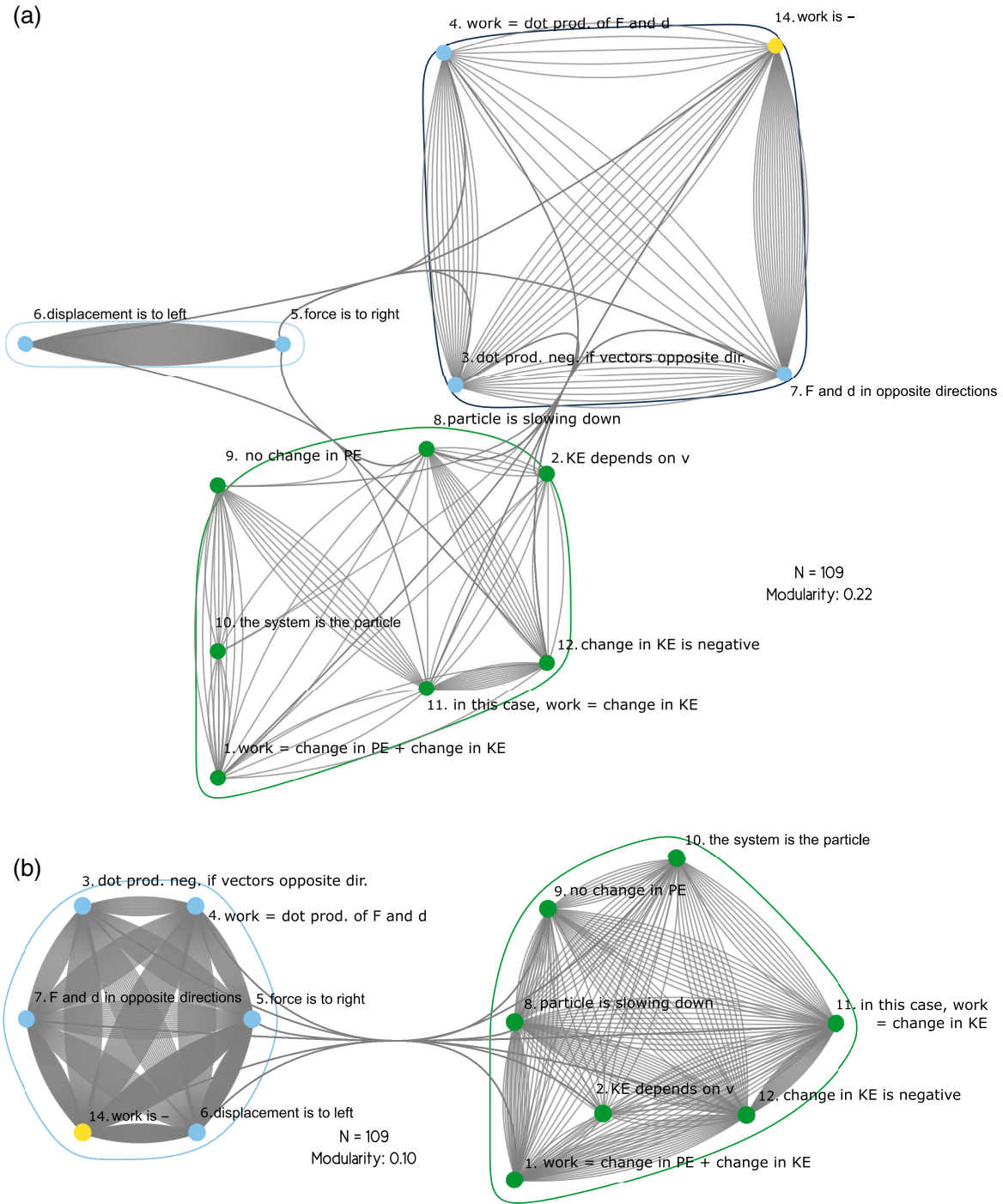
FIG. 5. A representation of the communities found in (a) a direct association network and (b) an indirect association network, both built from correct responses to the work-energy task described in Sec. IV. A. 2. Elements that are aligned with a work as dot-product argument are colored blue and the elements aligned with the work as a change in energy argument are colored green. The answer element is colored yellow. The modularity is given for reference. Note the especially dense connections between elements 5 and 6, suggesting a tight association between those elements in (a).
