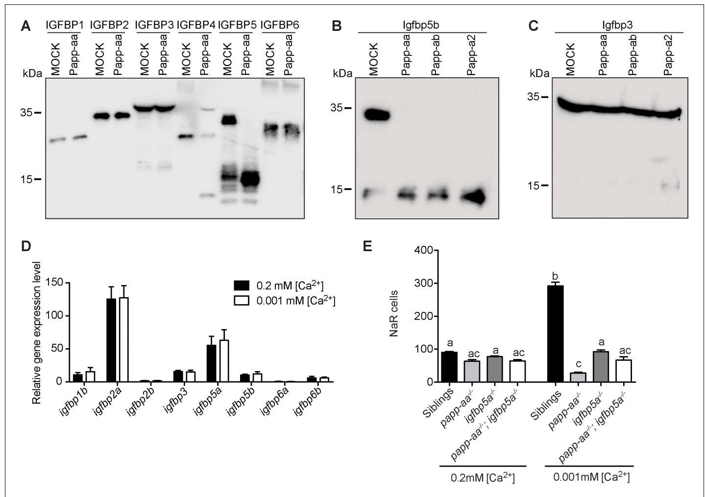
Figure 4. Papp-aa is an Igfbp5 proteinase and Papp-aa-mediated Igfbp5 proteolysis in NaR cells is critical. (A) Purified human IGFBP1, 2, 3, 4, 5, and 6 was incubated for 2 hr at 28°C with conditioned media collected from HEK293 cells transfected with zebrafish Papp-aa and from Mock transfected cells. For the IGFBP4 group, 100 nM IGF1 was added prior to the initiation of the proteinase assay. The protease reaction was stopped and analyzed by western blotting. (B) Conditioned media collected from HEK293 cells co-transfected with Igfbp5b and the indicated plasmid were analyzed by western blotting. Intact and cleaved Igfbp5b bands were indicated. (C) Conditioned media collected from HEK293 cells co-transfected with Igfbp3 and the indicated plasmid were analyzed by western blotting. Intact and cleaved Igfbp3 bands were indicated. (D) Tg(igfbp5a:GFP) fish were raised in E3 embryo medium to 3 days post fertilization (dpf) and transferred to embryo media containing the indicated [Ca 2+ ]. Eighteen hours later, NaR cells were isolated by FACS. The mRNA levels of the indicated igfbp genes were measured and shown. Data shown are Mean ± SEM, n = 4. (E) Progenies resulted from papp-aa +/- ; igfbp5a +/- and papp-aa +/- ; igfbp5a -/- intercrosses were raised in E3 embryo medium to three dpf and transferred to the normal [Ca 2+ ] (0.2 mM) or low [Ca 2+ ] (0.001 mM) embryo medium. At five dpf, NaR cells in each fish were labeled by igfbp5a mRNA expression and quantified. Each fish was genotyped individually afterward. Quantified data are shown. n = 18 ~ 63 fish/group. The online version of this article includes the following source data and figure supplement(s) for figure 4:
