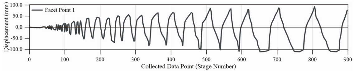
(a) Displacement Facet Point 1 near Base of Wall versus Stage Number
