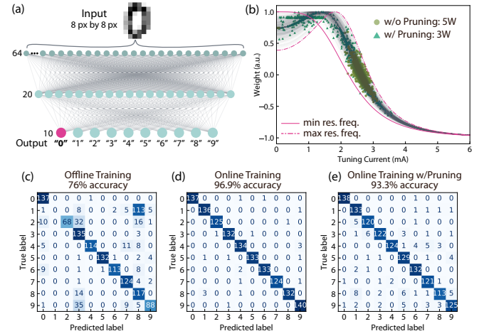
Fig. 2. Simulation on MNIST dataset. (a) PNN architecture has one hidden layer with 20 nodes fully connected to the input and output layers. (b) Weight tuning curves and trained current of all the 1480 MRRs. With pruning, the actuated tuning currents, shown as deep green triangles, are smaller than the non-pruning case, shown as light green dots. (c)-(e) Confusion matrix resulted from three training methods.
