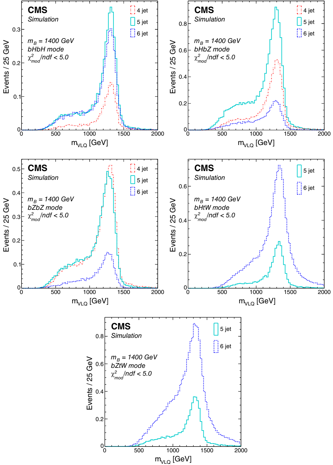
FIG. 3. Reconstructed VLQ mass distributions for simulated events for the channels in the fully hadronic category with m_B = 1400 \text{ GeV} . Upper row: channels in the bHbH (left) and bHbZ (right) decay modes. Middle row: channels in the bZbZ (left) and bHtW (right) decay modes. Lower row: channels in the bZtW decay mode. The different colors indicate the different jet multiplicities. A selection of \chi^2_{\text{mod}}/\text{ndf} < 5 has been applied. The values represent the expected number of events over the background in the 2016–2018 data sample.
