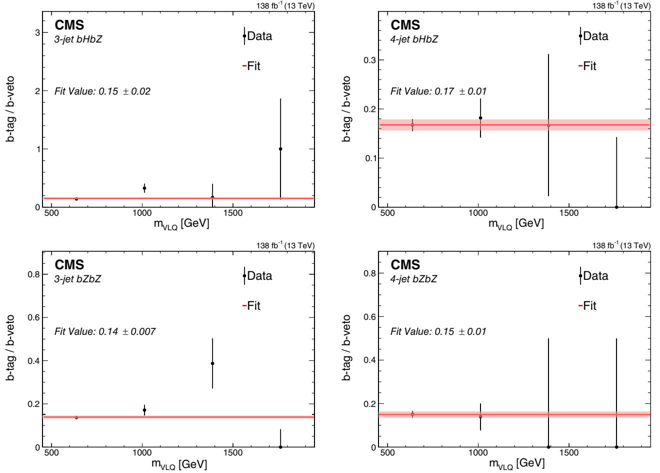
FIG. 10. Normalization factor as a function of m_{VLQ} for leptononic events in the 5 < \chi^2_{\text{mod}}/\text{ndf} < 20 region. Upper row: bHbZ events in the three-jet (left) and four-jet (right) channels. Lower row: bZbZ events in the three-jet (left) and four-jet (right) channels. The fit to a constant value and its uncertainty are shown by the red line and the light red shaded band, respectively.
