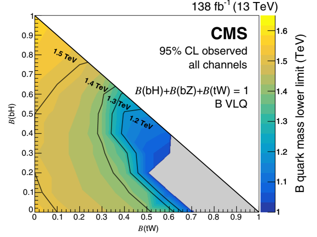
FIG. 20. Observed exclusion limits on the VLQ mass at 95% CL as a function of the branching fractions \mathcal{B}(B \rightarrow bH) and \mathcal{B}(B \rightarrow tW) , with \mathcal{B}(B \rightarrow tW) = 1 - \mathcal{B}(B \rightarrow bH) - \mathcal{B}(B \rightarrow bZ) . The gray area corresponds to the region where the exclusion limit is less than 1000 GeV.
