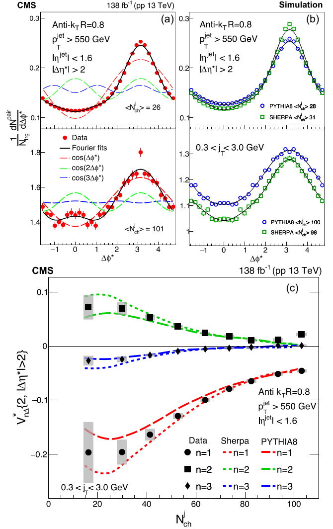
FIG. 3. Examples of two-particle angular correlations projected onto 1D \Delta\phi^* for |\Delta\eta^*| > 2 . The panels show (a) data and (b) PYTHIA8 and SHERPA for inclusive N_{\text{ch}}^j (upper) and high- N_{\text{ch}}^j (lower) jet selections. Data and both MC models are compared in (c) with a continuous evolution of extracted two-particle Fourier coefficients V_{n\Delta}^* as a function of N_{\text{ch}}^j . Vertical bars on data points indicate statistical uncertainty while shaded boxes represent systematic uncertainties. Projections are symmetrized about \Delta\phi^* = 0 and \pi .
