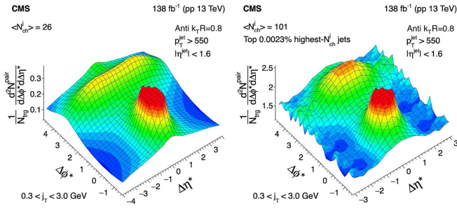
FIG. 2. Results for 2D two-particle angular correlation functions for particle 0.3 < j_T < 3.0 GeV from inclusive (left) and the highest (right) N_{\text{ch}}^j jets, for anti- k_T R=0.8 algorithm with p_T^{\text{jet}} > 550 GeV and |\eta^{\text{jet}}| < 1.6 .
