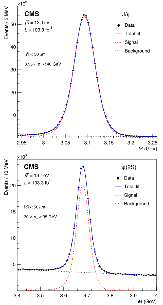
Fig. 4. Dimuon mass distributions measured for the prompt J/\psi (top) and \psi(2S) (bottom) event samples, in the mentioned p_T bins. The total fit function (blue), the sum of the two CB functions and (only in the J/\psi case) the Gaussian function (red), and the background continuum (black) are also shown.
