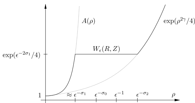
Fig. 2 When \epsilon > 0 is small, the weight W_\epsilon(R, Z) entering the energy functional (2.34) is close to a piecewise smooth radially symmetric function, which satisfies W_\epsilon \approx A(\rho) := (4/\rho^2)(e^{\rho^2/4} - 1) in the inner region where \rho := (R^2 + Z^2)^{1/2} \lesssim \epsilon^{-\sigma_1} . When W_\epsilon reaches the threshold value \exp(\epsilon^{-2\sigma_1}/4) , the weight is taken approximately constant until \rho = \epsilon^{-\sigma_2} , and outside that region we set W_\epsilon \approx \exp(\rho^{2\gamma}/4) with \gamma = \sigma_1/\sigma_2 . The dashed lines reflect the fact that \exp(\rho^{2\gamma}/4) \lesssim W_\epsilon \lesssim A(\rho) where the implicit constants do not depend on the parameter \epsilon . The intermediate scales \epsilon^{-\sigma_0} , where the truncation (2.28) occurs, and \epsilon^{-1} , which is the distance from the origin to the boundary \partial\Omega_\epsilon , are indicated for completeness
