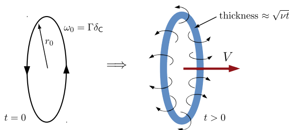
Fig. 1 An illustration our main result. Starting from a vortex filament supported on an oriented circle \mathbb{C} , the solution of the Navier-Stokes equation evolves into a viscous vortex ring of thickness proportional to \sqrt{\nu t} which moves along the symmetry axis at a speed V given by the Kelvin-Saffman formula (1.5). In the right picture, the vortex lines are circles that fill the depicted solid torus, whereas the curly arrows denote the trajectories of the fluid particles
