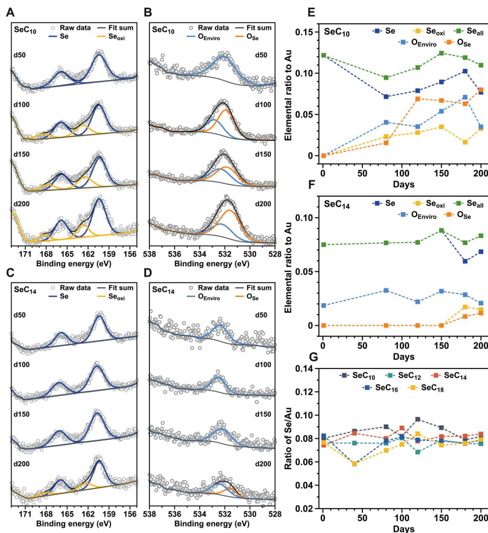
Fig. 4. The oxidation process of Au-SeC n monitored by XPS. (A) Se 3p peak spectrum for Au-SeC 10 . (B) O 1s peak spectrum for Au-SeC 10 . (C) Se 3p peak spectrum for Au-SeC 14 . (D) O 1s peak spectrum for Au-SeC 14 . The relative ratio of O and Se to Au from XPS Au-SeC 10 (E) and Au-SeC 14 (F) as a function of days. (G) Se/Au ratio of Au-SeC n ( n = 10, 12, 14, 16 , and 18 ) derived from XPS results as a function of days.
