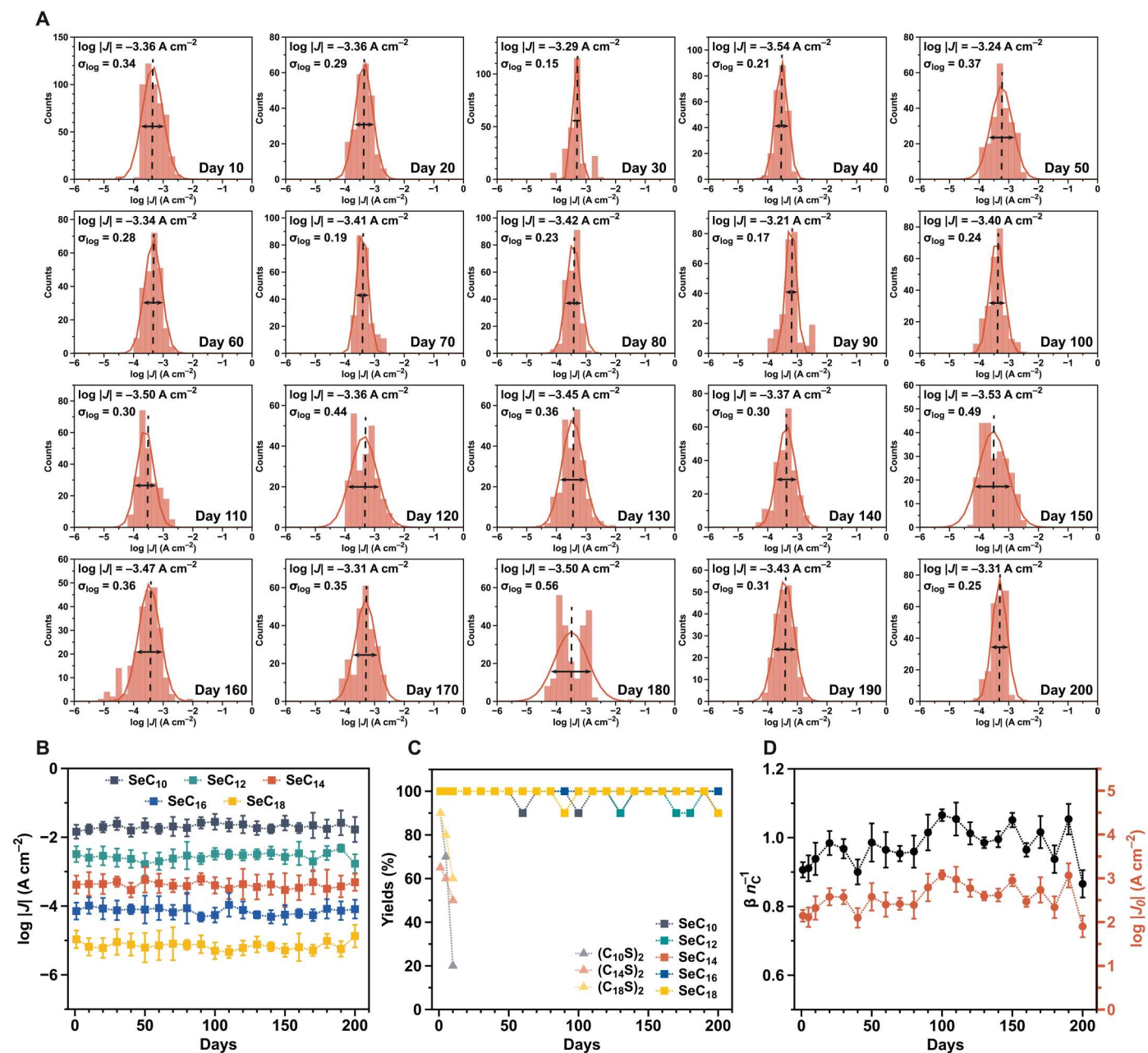
Fig. 3. The lifetime of Au-SeC n monitored by tunneling. (A) An example of the histograms of \log |J| at -0.50 V with Gaussian fits for all Au-SeC 14 /Ga 2 O 3 /EGaIn junctions measured every 10 days. (B) Plots of the \log |J| at -0.50 V for Au-SeC n /Ga 2 O 3 /EGaIn junctions as a function of days. (C) Yields of Au-SeC n /Ga 2 O 3 /EGaIn junctions as a function of days. n = 10, 12, 14, 16 , and 18 ; yields of Au-(C n S) 2 /Ga 2 O 3 /EGaIn junctions as a function of days. n = 10, 14 , and 18 . (D) Values of \beta and \log |J_0| measured as a function of days. All samples were kept under ambient conditions.
