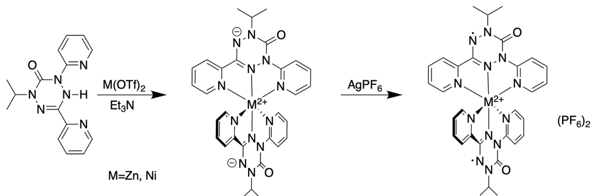
SCHEME 1 Synthesis of M(\text{dipyvd})_2 and [M(\text{dipyvd})_2](\text{PF}_6)_2 .
