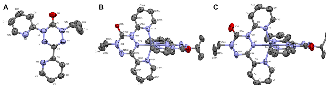
FIGURE 1 Thermal ellipsoid plots for (A) pyvdH, (B) Zn (dipyvd) 2 and (C) [Zn (dipyvd) 2 ](PF 6 ) 2 . Ellipsoids are drawn at 50% probability. For B only one of the two independent molecules in the unit cell is shown. For B and C the two ligands are related by symmetry; atomic labels for only one ligand are shown. Hydrogen atoms and PF 6 counterions are not shown for clarity.
