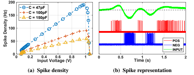
Figure 14: Characters of the spike encoding circuit.
