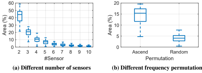
Figure 5: Localization ambiguity area with different settings.
