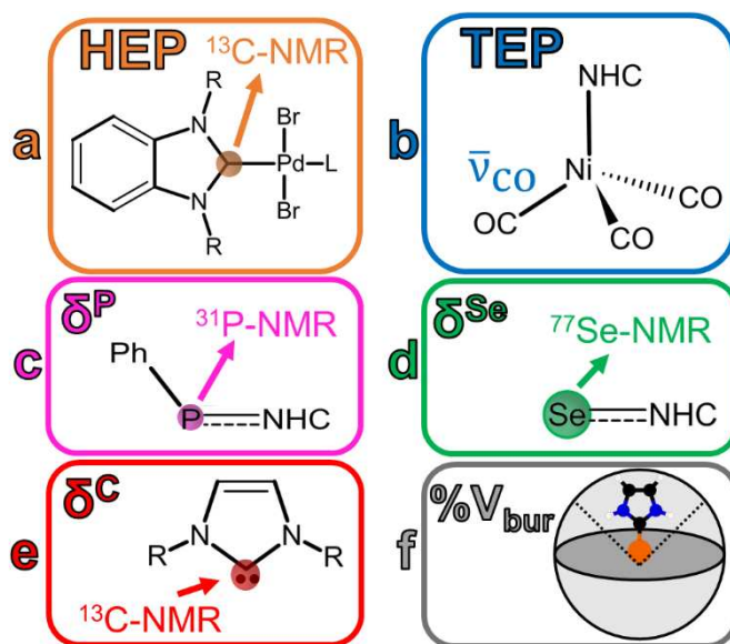
Figure 2: Schematic representations of (a/orange) the Huynh Electronic Parameter (HEP), (b/blue) the Tolman electronic parameter (TEP), (c/pink) phosphorous isotropic chemical shift ( \delta^{\text{P}} ), (d/green) selenium isotropic chemical shift ( \delta^{\text{Se}} ), (e/red) free-carbene carbon isotropic chemical shift ( \delta^{\text{C}} ), and (f/grey) percent buried volume ( \%V_{\text{bur}} ).
