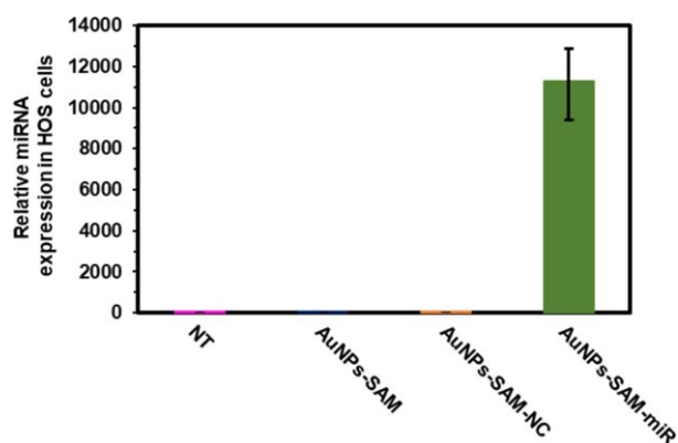
Figure 7. Relative miR-509-3p level in nontreated (NT) and AuNPs-SAM-, AuNPs-SAM-NC-, and AuNPs-SAM-miR-treated HOS cell lines measured by Taqman PCR.
