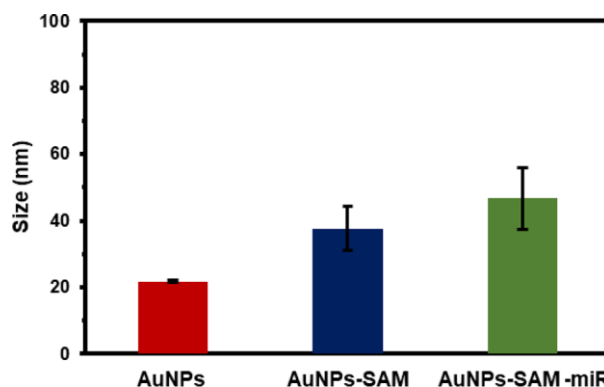
Figure 1. Hydrodynamic diameters of the AuNPs, AuNPs-SAM, and AuNPs-SAM-miR species, indicating average values of ~22, ~38, and
