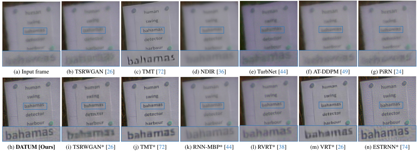
Figure 6. Qualitative comparison on the turbulence-text dataset [64]. The input frame (a) is the 49th frame of the 94th sequence in [64]. Figures on the top row are restoration results of corresponding TM methods using their original model and checkpoints. Figures on the bottom row are TM or general restoration models (marked by *) trained on our ATSyn-static dataset.
