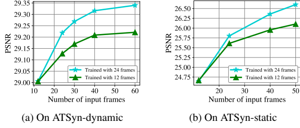
Figure 4. Influence of the number of input frames.
