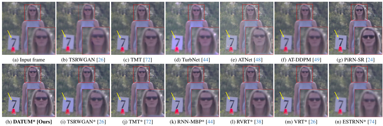
Figure 7. Qualitative comparison on a dynamic scene sample from the BRIAR dataset [16]. Figures on the top row are the original restoration results of corresponding TM methods. Figures on the bottom row are models (marked by *) trained on ATSyn-dynamic dataset.
