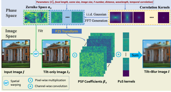
Figure 3. Scheme of our data synthesis method.
