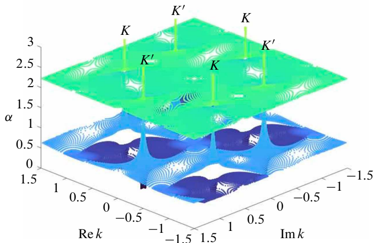
Figure 4. Dirac point dynamics for B = 0.1e^{2\pi i\theta} with \theta \in [0, 1/2] . Close to the first two magic angles ( \alpha \approx 0.585, 2.221 ), the dynamics spreads out in space.
