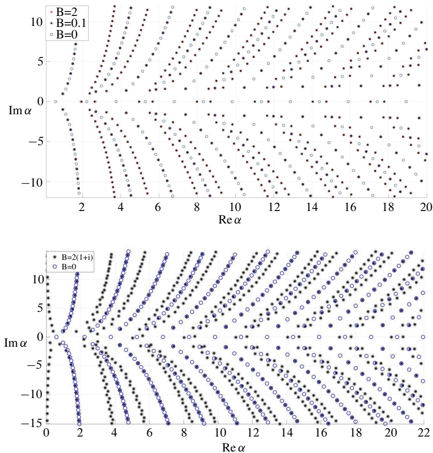
Figure 8. Top figure showing \alpha \in \mathbb{C} such that 1/\alpha \in \text{Spec}_{L_0^2}(T_K(B)) or K \in \text{Spec}_{L_0^2}(D_B(\alpha)) . We see that indeed for B \in \mathbb{R} \setminus \{0\} the trajectory of Dirac points passes through K, K' . Bottom figure showing \alpha \in \mathbb{C} such that 1/\alpha \in \text{Spec}_{L_0^2}(T_K(B)) or K \in \text{Spec}_{L_0^2}(D_B(\alpha)) . For general B \notin \mathbb{R} , the trajectory of Dirac points for varying \alpha \in \mathbb{R} does not pass through K between successive real magic angles.
