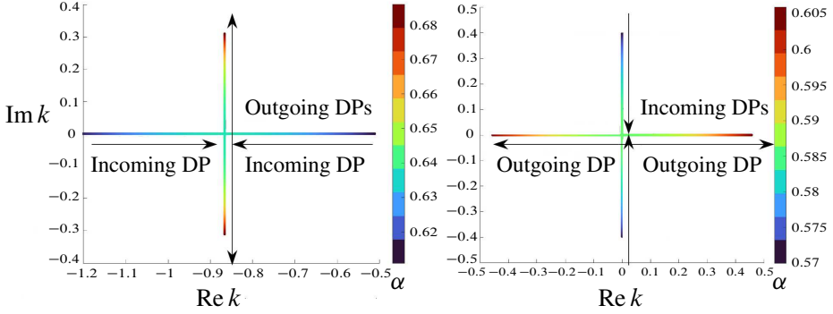
Figure 6. Bifurcation for B = 0.1 . (Top): the colour-coding indicates the position of the Dirac points for given values of \alpha \in \mathbb{R} . The right figure illustrates the bifurcation at \Gamma and the left figure at a non-equivalent (modulo \Lambda^* ) bifurcation point that is a vertex of the boundary of the Brillouin zone; see Figure 1.
