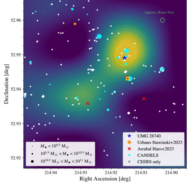
FIG. 3.— Overdensity hosting UMG-28740 (blue star) at z \sim 5 . The underlying 2D histogram and contours show the galaxy surface density for objects in the CANDELS catalog at 4.5 < z_{\text{phot}} < 5.5 and \log(M_\star/M_\odot) > 9 . The beam size (with a diameter of 4.5'' ) used to convolve the density map is shown in the upper right corner. Cyan circles denote photometric sources found in the CANDELS (Stefanon et al. 2017) and CEERS (Bagley et al. 2023) catalogs, where white circles are low-mass galaxies only found in the deeper CEERS catalog. The size of the circle indicates the estimated stellar mass of the object. Red crosses and the orange diamond are spectroscopically confirmed sources from Arrabal Haro et al. (2023a) and Urbano Stawinski et al. (2024b), respectively. The highlighted red cross indicates the location of the lower-mass member from Naidu et al. (2022).
