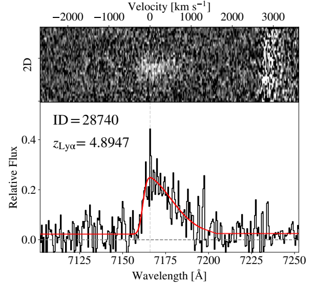
FIG. 1.— (top) A roughly 150 \text{ \AA} -wide section of the co-added 2D spectrum for UMG-28740 from our Keck/DEIMOS observations, highlighting the Lyman- \alpha emission line. (bottom) The corresponding co-added 1D spectrum with the resulting best-fit redshift shown in red. Top x-axis shows the velocity offsets from z_{\text{Ly}\alpha} while the bottom x-axis shows the observed wavelength.
