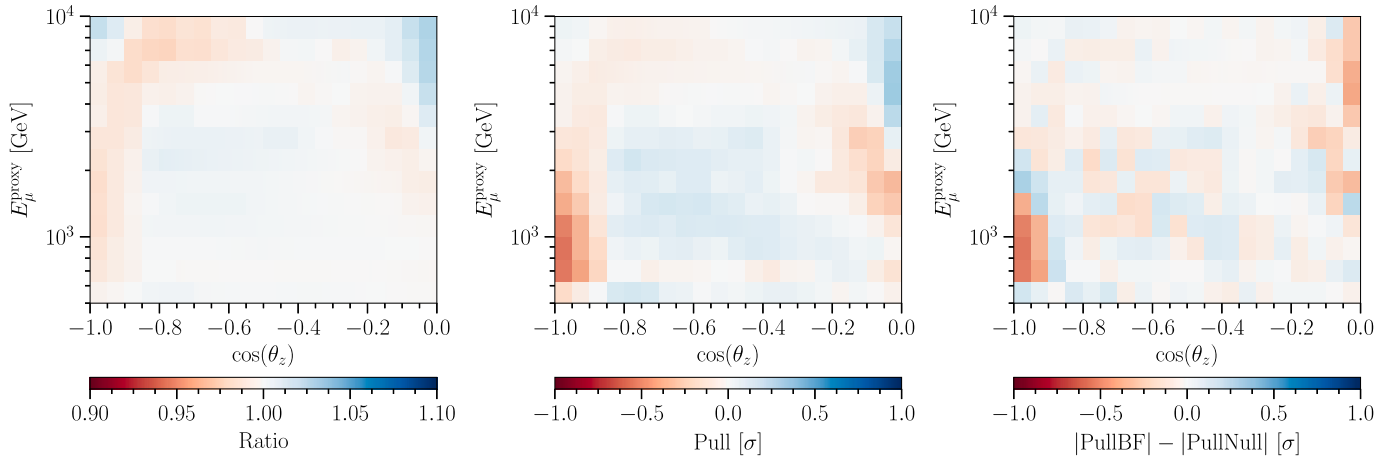
Fig. 4. Left: Ratio of the expected event rate for the best-fit hypothesis over the null hypothesis, bin-by-bin, in the \log_{10}(E) versus \cos(\theta_z) plane. Middle: Statistical pulls of the best-fit predicted event rate compared to the null expectation, bin-by-bin. Right: Difference between the absolute value of the pull of the data from the null hypothesis, and the absolute value of the pull of the data from the best-fit hypothesis. Red bins indicate where the data are in better agreement with the best-fit hypothesis, than with the null hypothesis; these are the bins driving the fit to the best-fit hypothesis point.
