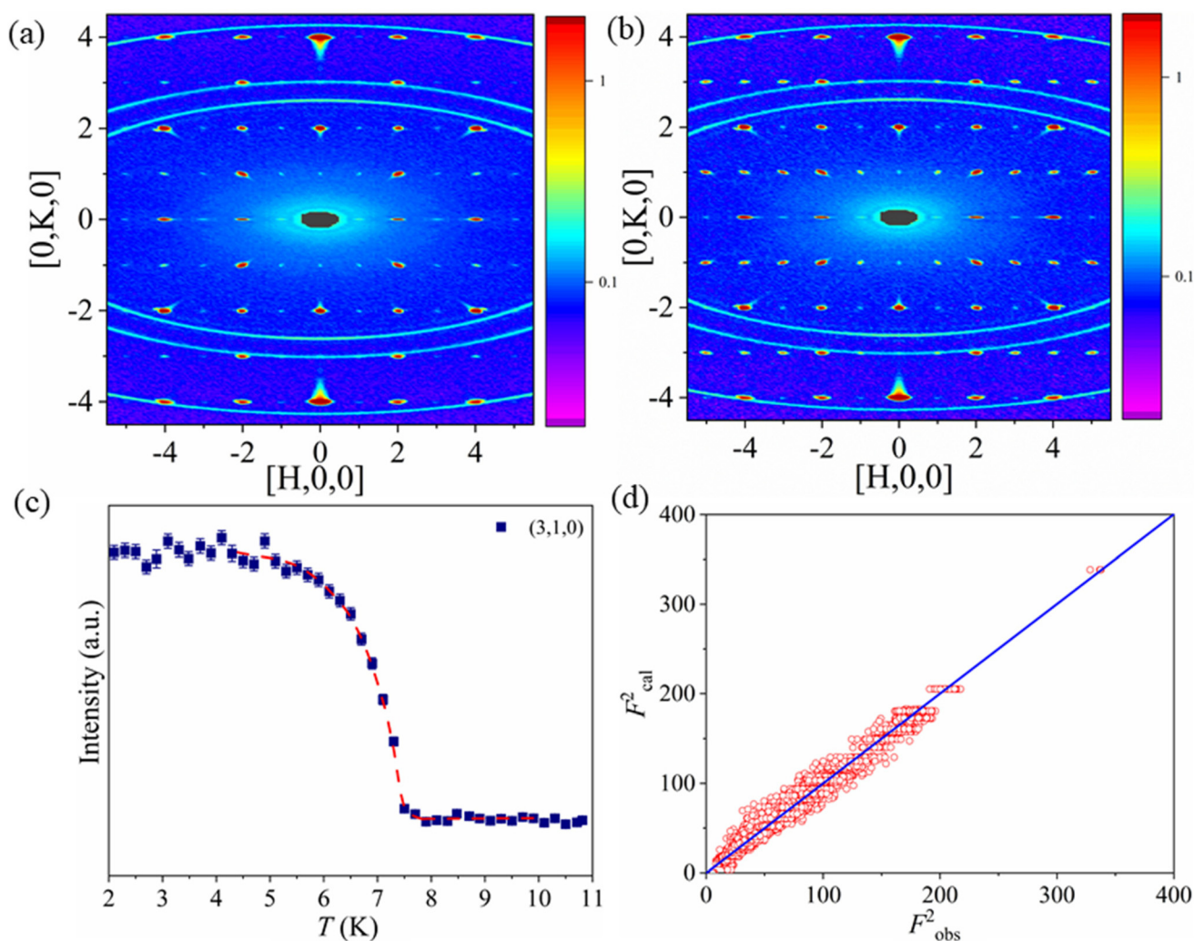
Fig. 4 (a) Data for the (HK0) plane at 15 K. (b) Data for the (HK0) plane at 1.5 K. (c) Temperature dependence of the (3,1,0) magnetic peak. (d) Single crystal of \text{K}_2\text{Co}_3(\text{MoO}_4)_3(\text{OH})_2 refinement of 1.5 K data showing the observed peak intensities versus the peak intensities of a calculated model.
