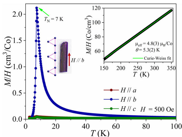
Fig. 2 Magnetic susceptibilities, \chi = M/H , of \text{K}_2\text{Co}_3(\text{MoO}_4)_3(\text{OH})_2 as a function of temperature under an applied field of 500 Oe along the three crystallographic axes. Inset: \text{K}_2\text{Co}_3(\text{MoO}_4)_3(\text{OH})_2 crystal highlighting the crystallographic b -axis (Co–O–Co chain axis) as the longest axis of the crystals. Temperature dependence of the inverse magnetic susceptibility \chi^{-1} in the temperature range 150 K–350 K. The solid line represents the Curie–Weiss fitting to the data from 150 to 350 K.
