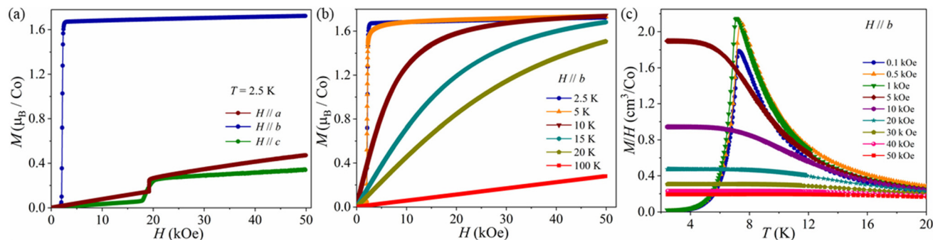
Fig. 3 (a) Isothermal magnetization data at 2.5 K along the three crystallographic axes. (b) The isothermal magnetization data along the b -axis within the temperature range of 2.5–100 K. (c) Field dependent magnetic susceptibility of \text{K}_2\text{Co}_3(\text{MoO}_4)_3(\text{OH})_2 measured in different magnetic fields along the b -axis ( H = 100 Oe–50 kOe) below 20 K.
