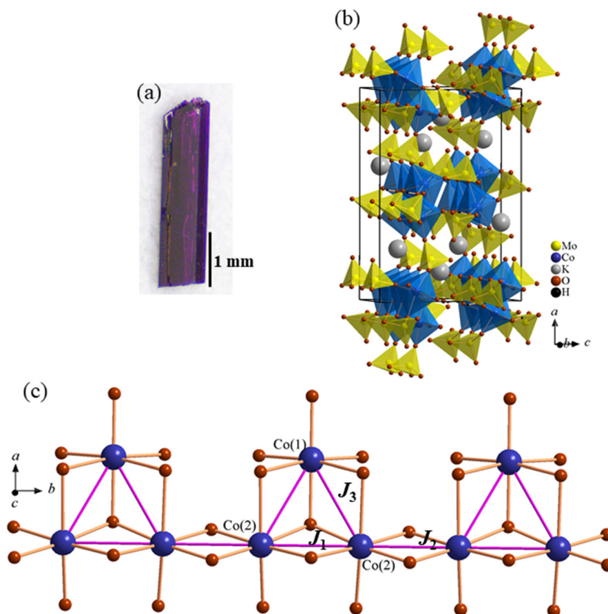
Fig. 1 (a) Hydrothermally grown single crystals of \text{K}_2\text{Co}_3(\text{MoO}_4)_3(\text{OH})_2 . (b) Partial polyhedral view of \text{K}_2\text{Co}_3(\text{MoO}_4)_3(\text{OH})_2 projected along the b -axis, showing packing of Co–O–Co half-sawtooth chains in the structure. The \text{K}^+ ions reside inside the cavities made by \text{CoO}_6 octahedron and \text{MoO}_4 tetrahedron. (c) Partial structure of Co–O–Co half-sawtooth chains made from edge-sharing \text{CoO}_6 octahedra along the b -axis. The unequal J_1 , J_2 and J_3 exchange interactions are shown using the solid pink line. The Co(2)–Co(2), J_1 , Co(2)–Co(2), J_2 , Co(1)–Co(2), J_3 , distances are 3.067(2), 3.017(2) and 3.226(2) Å, respectively.
