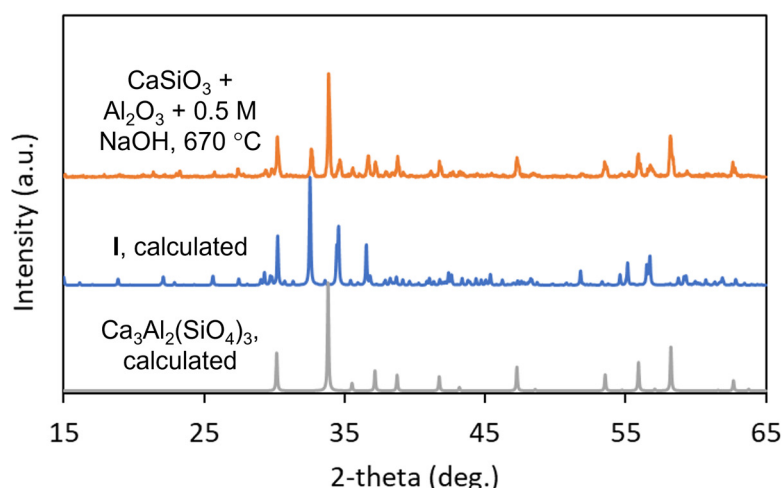
Figure 2. Powder X-ray diffraction pattern of the composite reaction product of \text{CaSiO}_3 + \text{Al}_2\text{O}_3 + 0.5 \text{ M NaOH} at 670^\circ\text{C} , indicating a mixture of the vesuvianite-type phase, I, and grossular garnet phase \text{Ca}_3\text{Al}_2(\text{SiO}_4)_3 .
