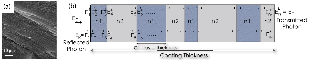
Fig. 1. (a) Layered snail shell structure made of calcite from scanning electron microscopy (SEM) image adapted from Parveen et al., 2020. For details, please refer to Ref. [3]. (b) Representation of multilayer coating with breakdown of electric field components in the multilayer, calculated using the transfer matrix formulation. Rightward moving electric field represents the transmitted component and left moving electric field represents the reflected component.
