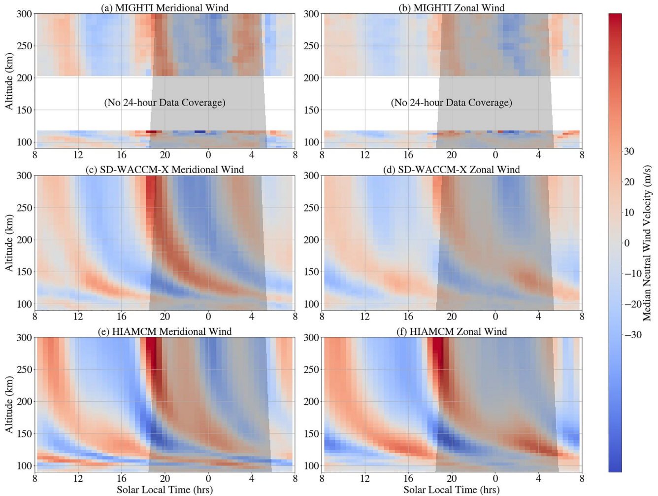
Figure 6. NH winter meridional (left) and zonal (right) winds averaged between 10° and 20° latitude as a function of altitude and SLT for (top) MIGHTI data (winter 2019 and 2020), (middle) SD-WACCM-X simulations (winter 2019 and 2020), and (bottom) HIAMCM simulations (15 January 2022). Diurnal tides have been removed. The gray shading shows the portion of the altitude/SLT space that is in darkness. Northward and eastward winds are defined to be positive.
