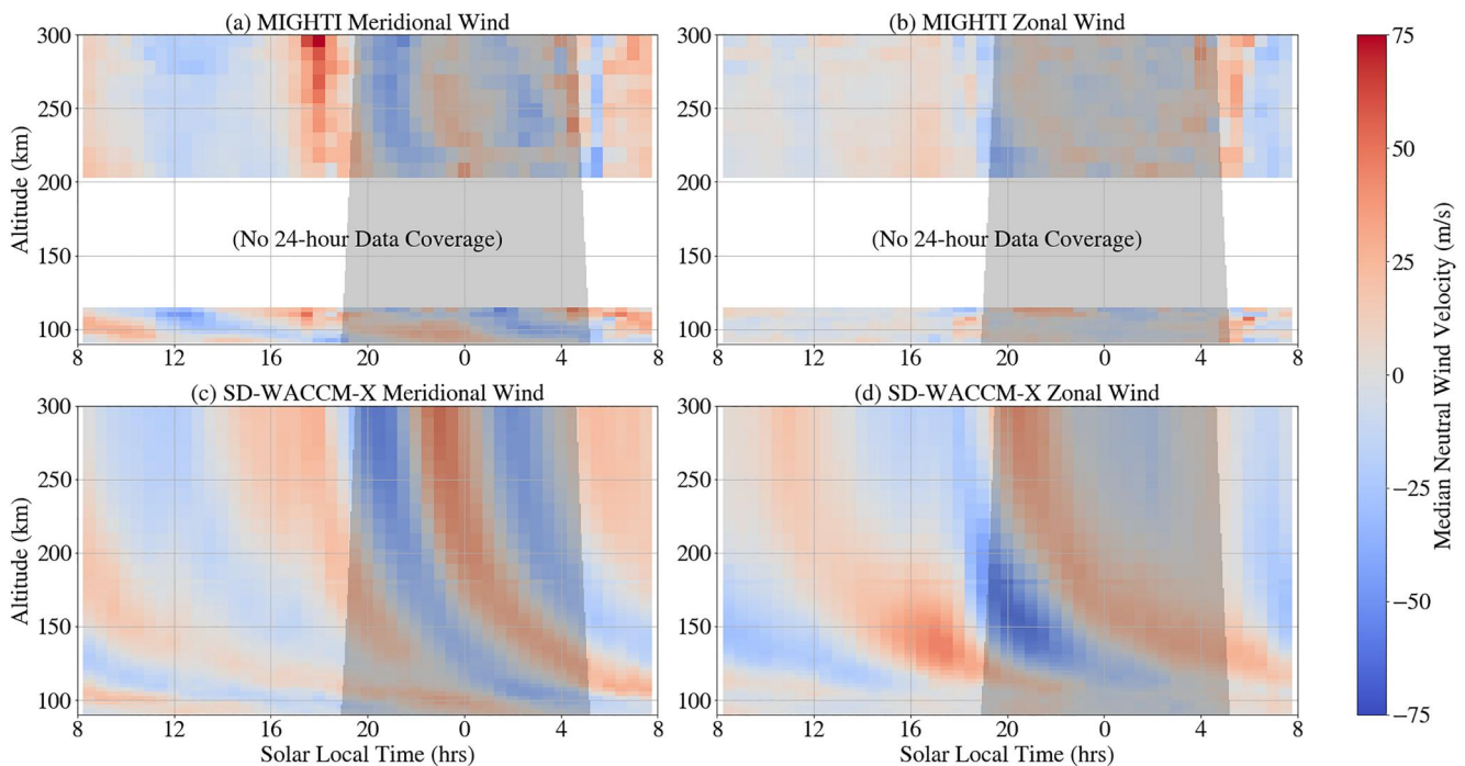
Figure 7. NH summer meridional (left) and zonal (right) winds averaged between -10^{\circ} and 0^{\circ} latitude as a function of altitude and SLT for (top) MIGHTI data (winter 2019 and 2020), (bottom) SD-WACCM-X simulations (winter 2019 and 2020). Diurnal tides have been removed. The gray shading shows the portion of the altitude/SLT space that is in darkness. Northward and eastward winds are defined to be positive.
