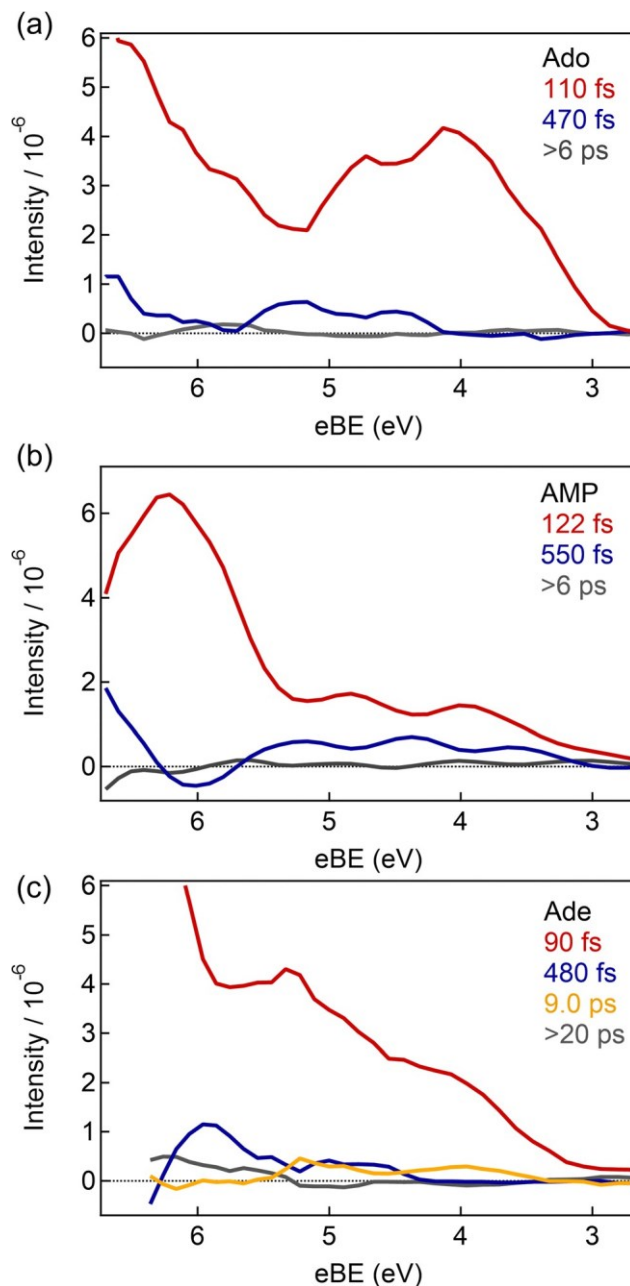
Fig. 6 DASs obtained from GLA for (a) Ado, (b) AMP, and (c) Ade. t_i for each DAS i is shown in the same color on the top right. The gray spectra represent the long-lived offset (c).
