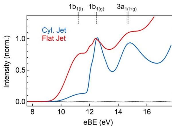
Fig. 3 One photon photoelectron spectra of an aqueous Ado solution depending on the mode of a jet; a 30-mm cylindrical jet (blue) and a flat jet (red).
