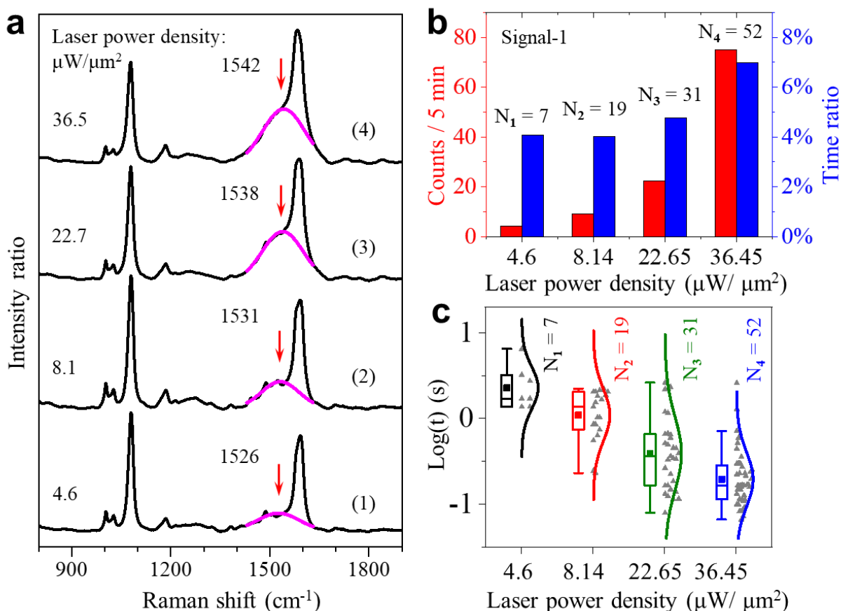
Fig. 3 (a) Four representative SERS average spectra under four different laser power densities. The pink lines are the Gaussian fits to the broad peaks near 1531 \text{cm}^{-1} . (b) Appearance event counts (red) and total appearance time percentage (blue) for signal-1 under different laser power densities. (c) Lifetime of signal-1 in logarithmic scale under four different laser power densities.
