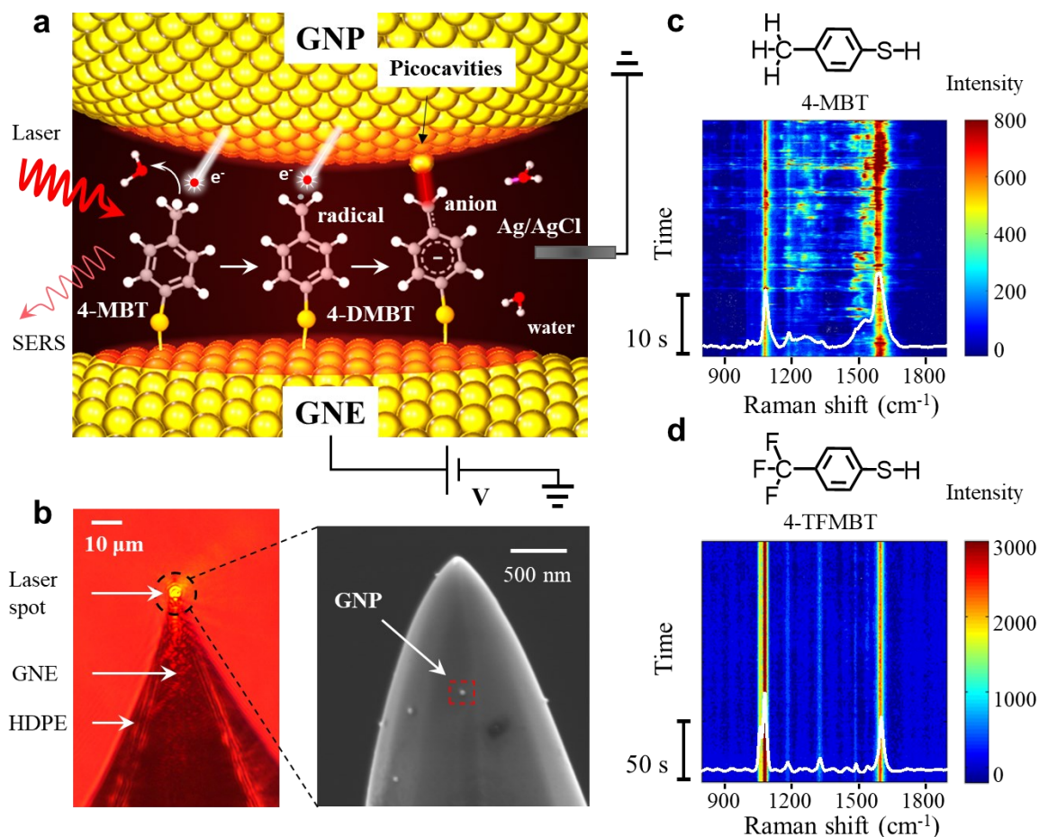
Fig. 1 (a) SERS experimental setup and the schematic representation of the plasmon mediated reaction of the 4-MBT molecules in the GNE-GNP junctions, sequentially resulting in benzyl radical and anion. (b) Left, optical microscope image of a HDPE insulated GNE with the laser beam focusing on the apex. Right, SEM image of a 4-MBT modified GNE apex (without HDPE coating) with attached GNPs. (c-d) Representative SERS time trajectory of 4-MBT (c) and 4-TFMBT (d).
