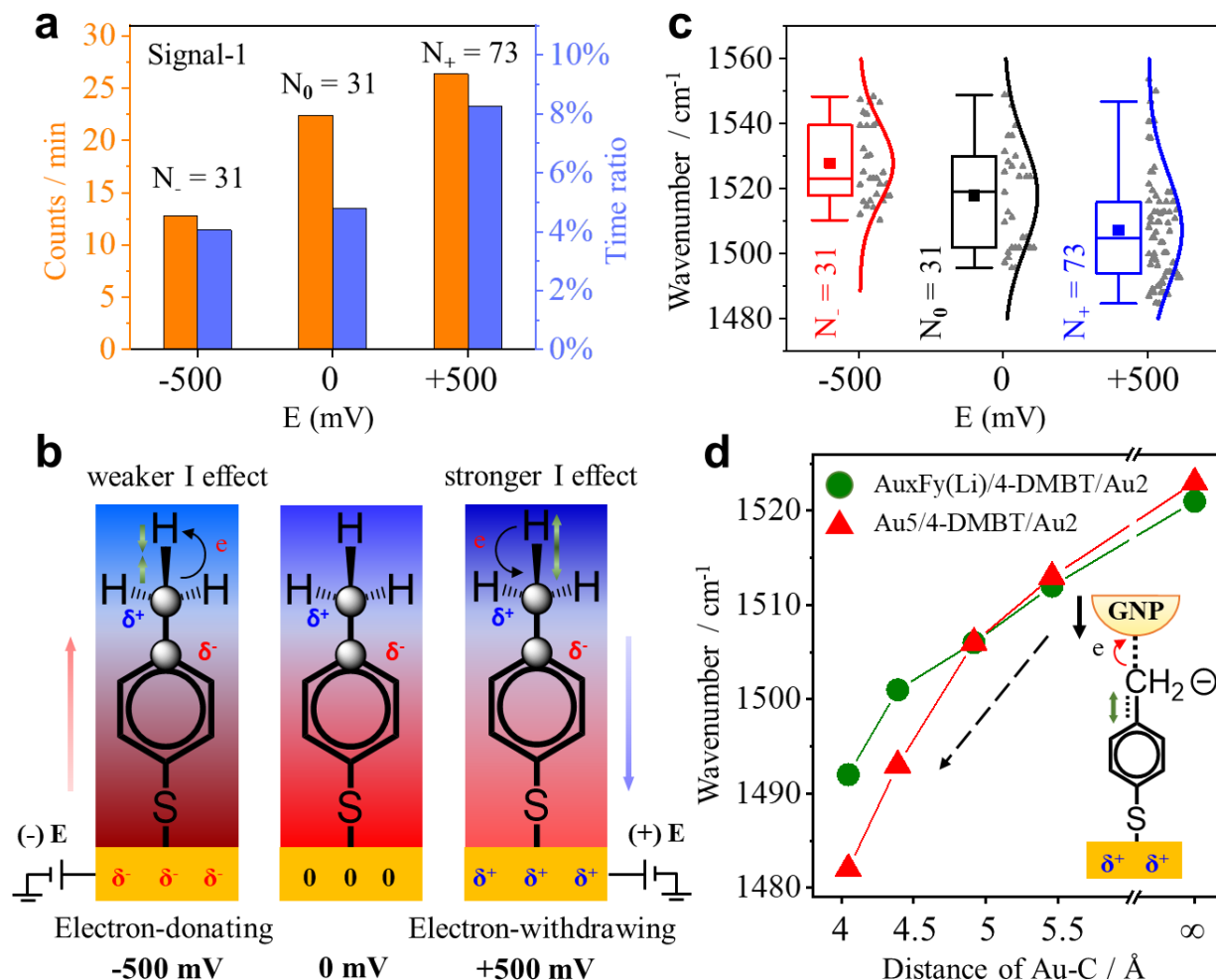
Fig. 5 (a) Occurrence rate (orange column) and appearance time ratio (blue column) under different E s. (b) Illustrations of the change in the strength of the I effect and in the bond length of the associated chemical bonds. The charge distribution for 4-MBT under different E s is also shown. The blue shades represent the positive group and the red represents the negative group. From left to right, the electronegativity of the phenyl group decreases. The green arrow indicates the change in C-H bond length. The black arrow shows the direction of the electron cloud shift. (c) Box plots for the position of the peak near 1530 \text{cm}^{-1} of signal-1 under different E s with the raw data (gray dots) in scatter plots. The solid lines are the Gaussian fits. The solid square dots represent the mean values of the wavenumber. N is the total number of events under
