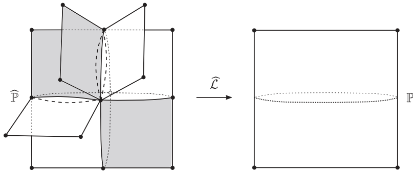
FIGURE 13. A branched covering map \widehat{\mathcal{L}}: \widehat{\mathbb{P}} \rightarrow \mathbb{P} induced by the flapped pillow \widehat{\mathbb{P}} on the left.
