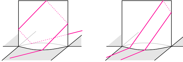
FIGURE 17. A pullback \widehat{\gamma} going over a horizontal flap in \widehat{\mathbb{P}} .
