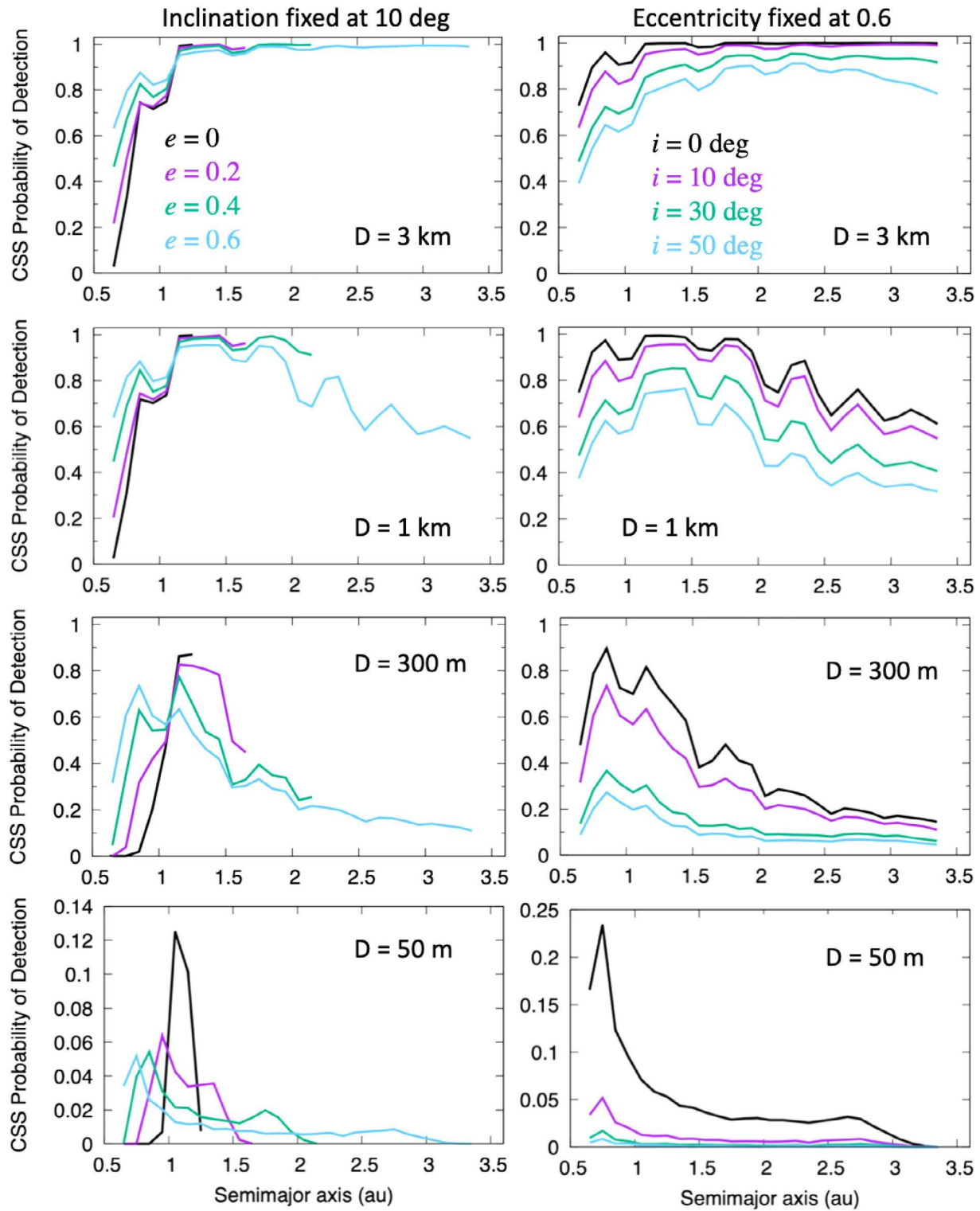
Fig. 7. The CSS2 detection probability (Eq. (7)) as a function of orbital elements for four different absolute magnitude values. From top to bottom, we plot P(a, e, i, H) for H corresponding to objects with D = 3 \text{ km} , 1 \text{ km} , 300 \text{ m} and 50 \text{ m} (for the reference albedo p_v = 0.14 ). The plots in the left column show P for the fixed orbital inclination ( i = 10^\circ ) and several eccentricity values. The plots on the right show P for e = 0.6 and several inclination values. The detection probability was computed for orbits with q < 1.3 \text{ au} .
