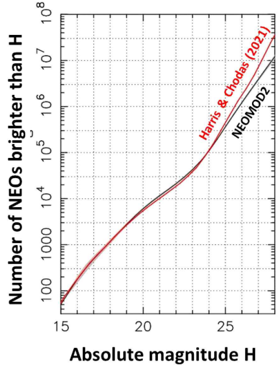
Fig. 12. The intrinsic (debiased) absolute magnitude distribution of NEOs from our base model (black line is the median) is compared to the magnitude distribution from Harris and Chodas (2021) (red line). The gray area is the 3\sigma envelope obtained from the posterior distribution computed by MultiNest. It contains – by definition – 99.7% of our base model posteriors. (For interpretation of the references to color in this figure legend, the reader is referred to the web version of this article.)
