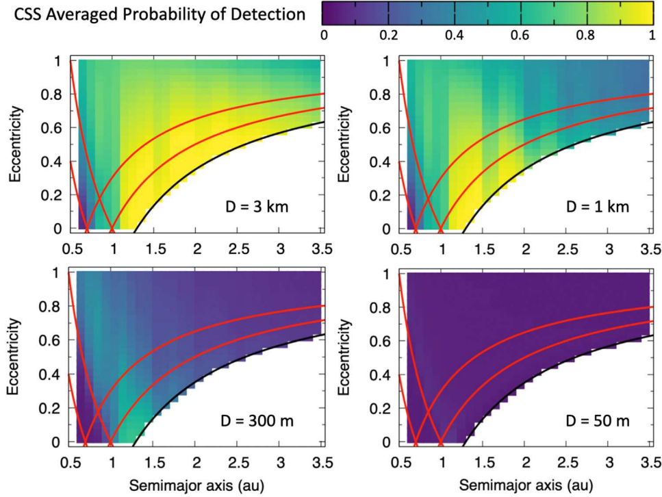
Fig. 6. The CSS2 detection probability (Eq. (7)) as a function of orbital elements for four different absolute magnitude values. From top-left to bottom-right, we plot P(a, e, i, H) for H corresponding to objects with D = 3 km, 1 km, 300 m and 50 m (for the reference albedo p_V = 0.14 ). The detection probability was averaged over all inclinations bins. The vertical strips, with P going up and down as a function of NEO's semimajor axis, are a consequence of the synodic effect (see discussion in Paper I). The red lines show borders of the orbital domain where orbits can have close encounters with Earth and Venus.
