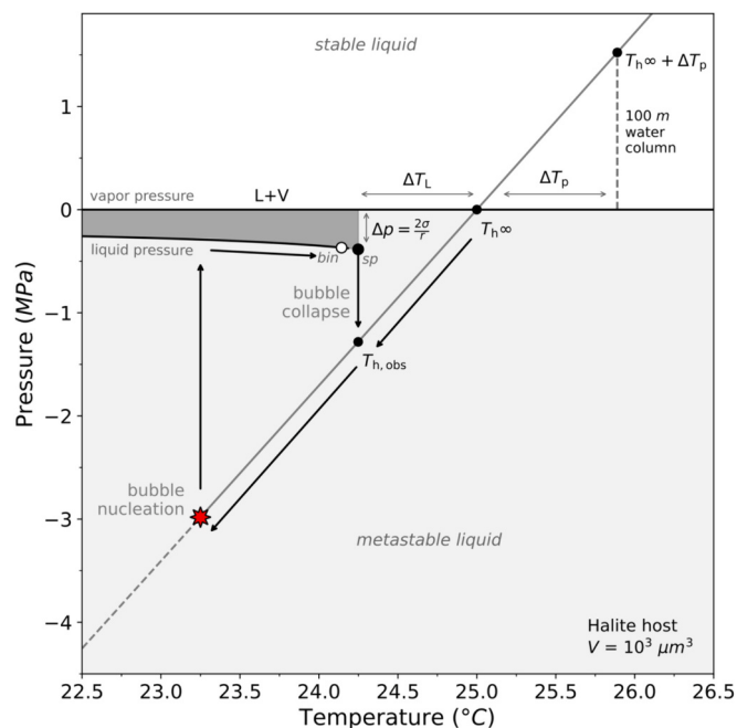
Fig. 6. p - T diagram of NaCl-saturated water illustrating the change in liquid pressure for single- and two-phase states as a function of temperature for a 1000\ \mu\text{m}^3 inclusion with T_h^\infty of 25.0\ ^\circ\text{C} , as well as the Laplace- and hydrostatic-pressure corrections for an inclusion in halite formed at 100\ \text{m} water depth (Modified from Krüger et al., 2011). Upon vapor bubble nucleation, liquid pressure increases but remains negative (tension), while vapor pressure is close to saturation pressure, resulting in a pressure difference \Delta p (Laplace pressure). Upon heating, the vapor bubble becomes smaller and \Delta p increases according to the Young-Laplace equation (as shown). At temperature T_{\text{bin}} , the stable two-phase state becomes metastable ( binodal ) and finally mechanically unstable at T_{\text{sp}} ( spinodal ). Bubble collapse is observed at T_{h,\text{obs}} , between T_{\text{bin}} and T_{\text{sp}} , so a Laplace correction term \Delta T_L is needed to account for the difference between T_{h,\text{obs}} and T_h^\infty . If the inclusion was trapped at the bottom of a water column, a hydrostatic pressure correction \Delta T_p is needed to account for the difference between saturation ( T_p^\infty ) and hydrostatic pressure.
