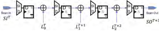
Fig. 4. Example of scan chain modeling with N = 3 at any clock cycle T . The scan out is denoted as SO^{T+3} = SI^T \oplus L_0^T \oplus L_1^{T+1} \oplus L_2^{T+2} .
