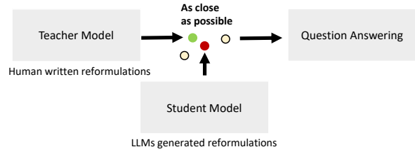
Figure 2: Reformulation imitator.
