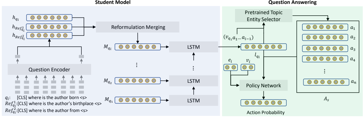
Figure 1: Training Process of CORNNET. The light gray part denotes the architecture of the student model. The light green part shows the framework of RL-based question answering model. Both are trained end-to-end.
