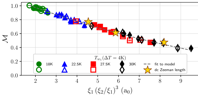
FIG. 3. The data from Fig. 2 collapse as a function of memory loss modeled in Eq. (4). Additionally, the three starred data points use correlation lengths extracted from dc experiments with the ac values of memory. T_{w_1} (18, 22.5, 27.5, and 30 K) and T_{w_1} - T_{w_2} = 4 \text{ K} . In both cases either the first (closed markers) or second (open markers) waiting times are varied from 0 to 6 hours, while the other waiting time is fixed at 3 (1) hours.
