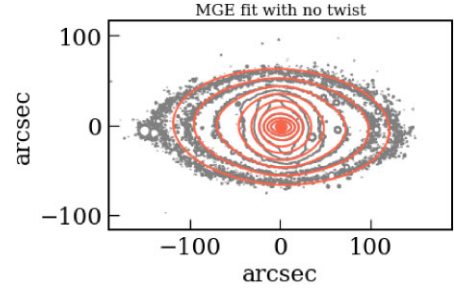
Figure A1. The contours of the NGC 4371 S4G image (grey), overlaid with contours of the best-fitting MGE (red) without twist between different Gaussians applied to the whole galaxy.
