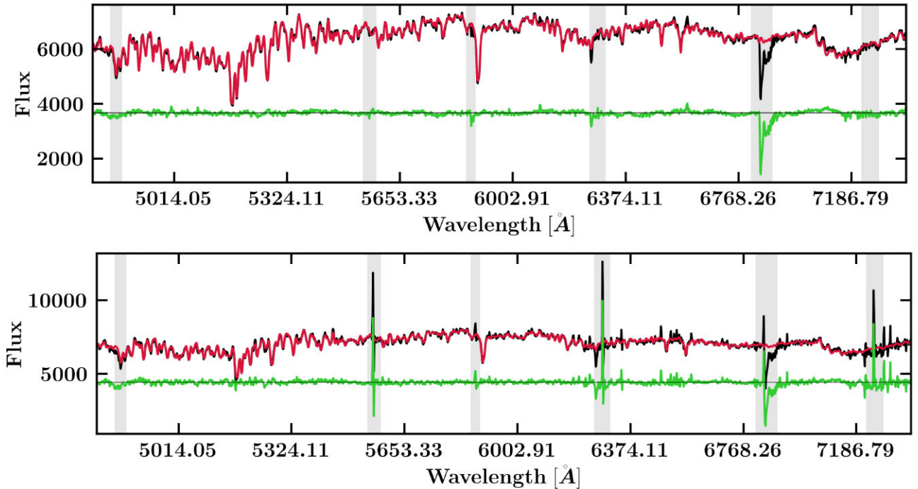
Figure 1. Integrated MUSE spectra (black line) and PPXF fits of NGC 4371 (red lines) are shown for two Voronoi bins, one from the central region (top) and one from the outer region (bottom). The spectra are plotted over the wavelength range of 4800–7300 Å, fitted to the MILES stellar templates. The residuals between the observed spectrum and the best-fitting model are displayed as a green line. Grey-shaded areas indicate regions that were masked during the fit, often due to emission lines or insufficient sky subtraction.
