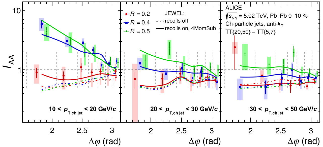
FIG. 3. I_{AA}(\Delta\phi) for R = 0.2, 0.4 and 0.5 , for intervals in recoil p_{T, \text{ch jet}} : [10, 20] , [20, 30] , and [30, 50] GeV/c. The central points and systematic uncertainties are offset from the center of the \Delta\phi intervals for clarity. The vertical dashed gray lines represent the \Delta\phi interval edges. Predictions from JEWEL are also shown.
