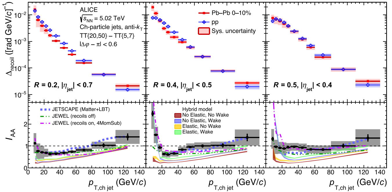
FIG. 1. Distributions of recoil jets with R = 0.2, 0.4 , and 0.5 in pp and central Pb-Pb collisions at \sqrt{s_{\text{NN}}} = 5.02 TeV. Upper panels: corrected \Delta_{\text{recoil}}(p_{\text{T, ch jet}}) distributions. Lower panels: I_{\text{AA}}(p_{\text{T, ch jet}}) (see text). Also shown are calculations based on JETSCAPE [16], JEWEL [34,35], and the Hybrid model [40].
