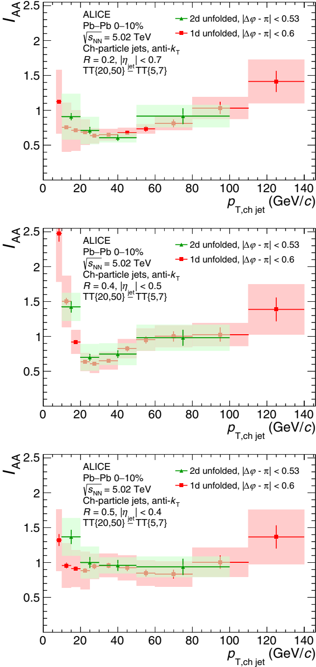
FIG. 22. I_{AA}(p_{T, \text{ch jet}}) from the \Delta_{\text{recoil}}(p_{T, \text{jet}}) distributions and \Delta_{\text{recoil}}(\Delta\varphi) distributions projected within similar \Delta\varphi intervals, measured for R = 0.2 (top), 0.4 (middle), and 0.5 (bottom) in central Pb-Pb and pp collisions.
