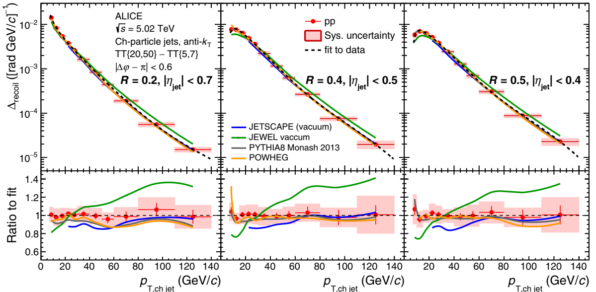
FIG. 11. (upper panels) corrected \Delta_{\text{recoil}}(p_{T,\text{ch,jet}}) distributions measured for R = 0.2 (left), 0.4 (middle), and 0.5 (right) in pp collisions at \sqrt{s} = 5.02 TeV, compared with calculations from JETSCAPE [110], JEWEL [115,116], PYTHIA8 [99,100], and POWHEG [102–105]. (lower panels) Ratio of the data and calculations to a functional fit of the measured \Delta_{\text{recoil}}(p_{T,\text{ch,jet}}) distributions.
