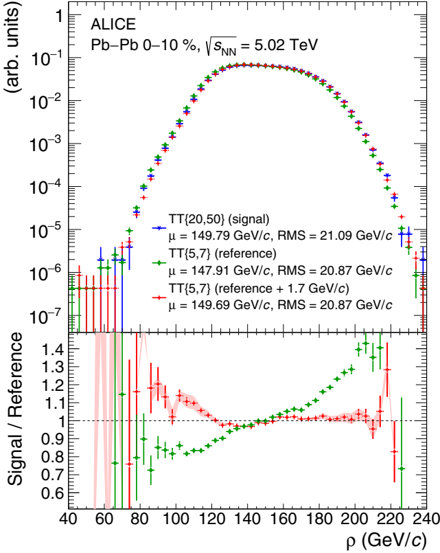
FIG. 2. \rho distributions for central Pb-Pb collisions at \sqrt{s_{NN}} = 5.02 TeV. (upper panel) TT_{sig} and TT_{ref} distributions, and the TT_{ref} distribution shifted by \Delta\rho = 1.7 GeV/c (Sec. IV A). (lower panel) Ratio of TT_{ref} and shifted TT_{ref} to TT_{sig} distribution. The mean \mu and RMS of the distributions are given in the legend. The vertical lines on the data points are the statistical uncertainties, and the shaded band on the ratio of the TT_{sig} over the shifted TT_{ref} distributions represents the systematic uncertainty of the procedure.
