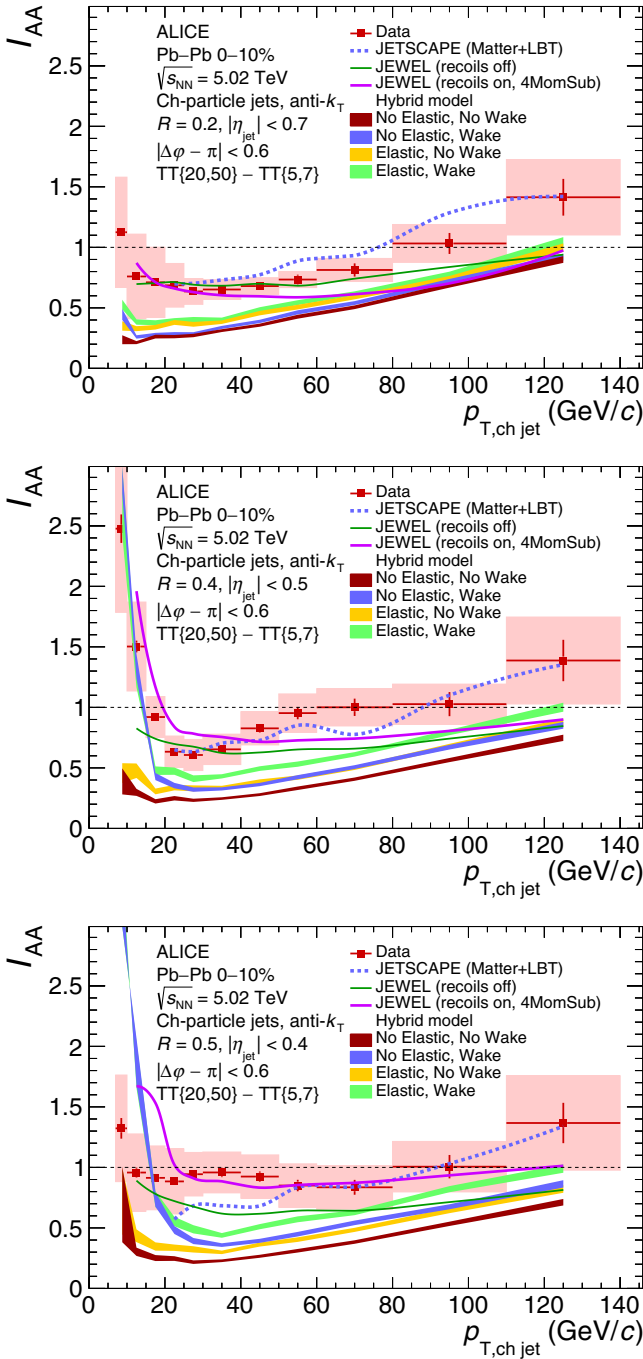
FIG. 15. I_{AA}(p_{T,ch jet}) from the \Delta_{recoil}(p_{T,jet}) distributions measured for R = 0.2 (top), 0.4 (middle), and 0.5 (bottom) in central Pb-Pb (Fig. 13) and pp collisions (Fig. 11). JETSCAPE, JEWEL, and the Hybrid Model calculations are also shown.
