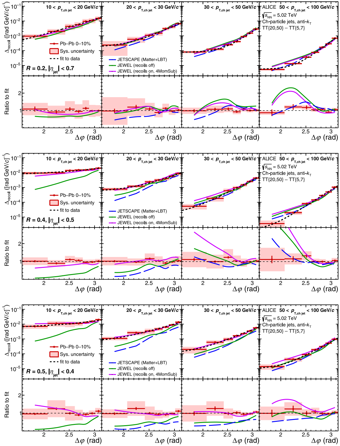
FIG. 14. Corrected \Delta_{\text{recoil}}(\Delta\phi) distributions for Pb-Pb collisions at \sqrt{s_{\text{NN}}} = 5.02 TeV, for R = 0.2 (top), 0.4 (middle), and 0.5 (bottom) in p_{\text{T, ch jet}} bins (left to right): [10, 20] , [20, 30] , [30, 50] , and [50, 100] GeV/c. JETSCAPE and JEWEL calculations are also shown. Upper subpanels show the individual distributions, while lower subpanels show their ratio to a functional fit of the data.
