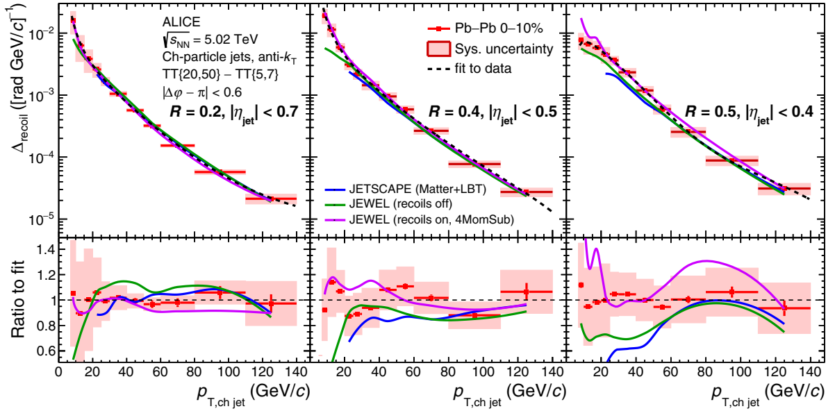
FIG. 13. (upper panels) Corrected \Delta_{\text{recoil}}(p_{T, \text{ch jet}}) distributions measured for R = 0.2 (left), 0.4 (middle), and 0.5 (right) in Pb-Pb collisions at \sqrt{s_{\text{NN}}} = 5.02 TeV, compared with theoretical calculations from JETSCAPE and JEWEL. (lower panels) Ratio of the data and calculations to a functional fit of the measured \Delta_{\text{recoil}}(p_{T, \text{ch jet}}) distributions.
