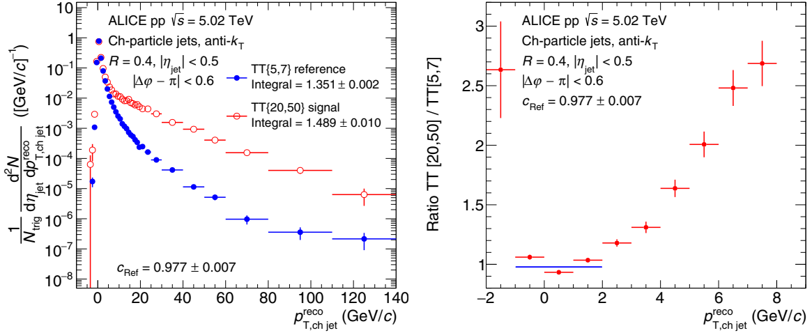
FIG. 7. (left) Trigger-normalized semi-inclusive recoil jet distributions with R = 0.4 for TT sig - and TT ref -selected populations in pp collisions at \sqrt{s} = 5.02 TeV. (right) Ratio of the two distributions. The horizontal blue line indicates the fit to the ratio close to p_{T,\text{ch jet}}^{\text{reco}} = 0 for the determination of c_{\text{Ref}} , the value of which is also given in the figures.
