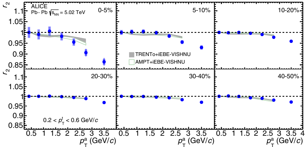
FIG. 5. The factorization ratio r_2 for Pb–Pb collisions at \sqrt{s_{NN}} = 5.02 TeV (blue circles) as a function of p_T^a for 0.2 < p_T^T < 0.6 GeV/c. The different panels display results in different centrality intervals. Statistical (systematic) uncertainties are represented by solid bars (faded boxes). Predictions from iEBE-VISHNU hydrodynamic model with T_REnto initial conditions and temperature-dependent \eta/s(T) [71], and with AMPT initial conditions and \eta/s = 0.08 [71], are shown in colored bands.
