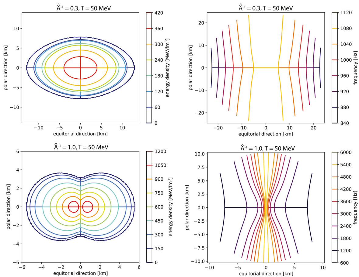
FIGURE 6 Energy density (left) and frequency (right) contours for individual stellar models at two degrees of differential rotation, constructed using the EOS model at T = 50 MeV. The top row has a lower degree of differential rotation ( \hat{A}^{-1} = 0.3 ) and the bottom has a higher degree ( \hat{A}^{-1} = 1.0 ).
