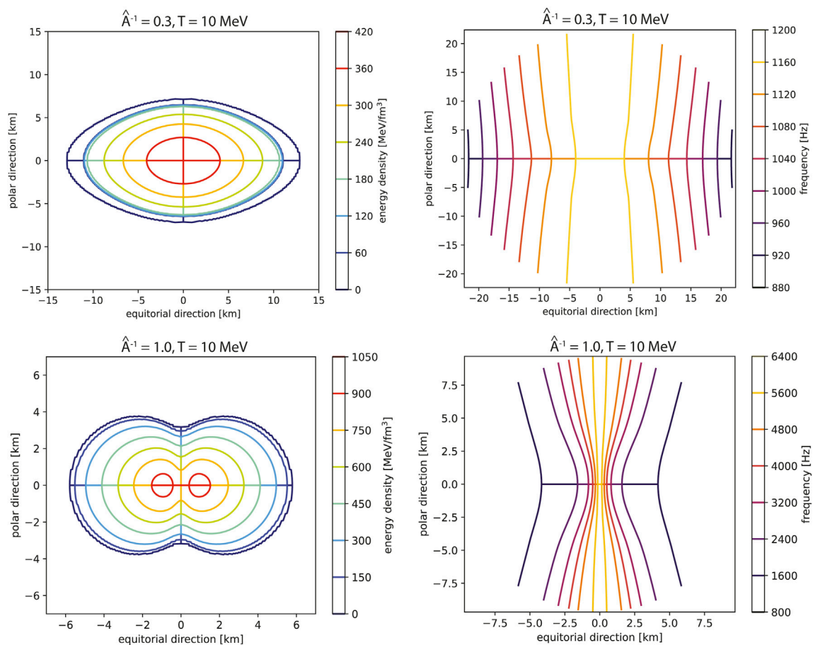
FIGURE 5 Energy density (left) and frequency (right) contours for individual stellar models at two degrees of differential rotation, constructed using the EOS model at T = 10 MeV. The top row has a lower degree of differential rotation ( \hat{A}^{-1} = 0.3 ) and the bottom has a higher degree ( \hat{A}^{-1} = 1.0 ).
