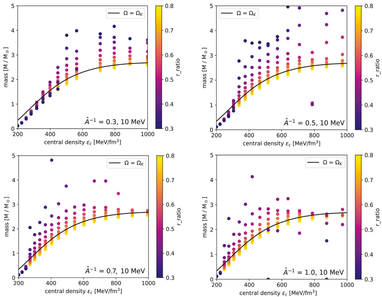
FIGURE 2 Mass vs. central density of sequences of differentially rotating neutron stars constructed using the EOS model at T = 10 MeV. The four panes show values for four instances of the rotation parameter \hat{A}^{-1} over a range of central densities and r_{ratio} values compared to a sequence of uniformly rotating stars at the respective Kepler limit (see text for more details).
