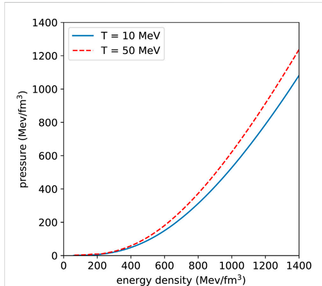
FIGURE 1 Pressure as a function energy density for the two EOS models at T = 10 and 50 MeV.
