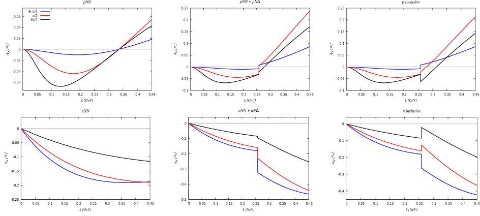
Figure 3: A_N vs k with no form factors and stable \Delta . Top (bottom) panels proton (neutron). Left: elastic with only nucleon in the TPE amplitude, middle: elastic with nucleon and \Delta in TPE amplitude, right: inclusive.
