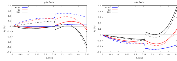
Figure 5: Inclusive A_N for proton (left panel) and neutron target (right panel). Comparison between the LO in 1/N_c (dashed lines) and the results of this work (solid lines). Form factors are included, and the physical phase space is used in the LO result.
