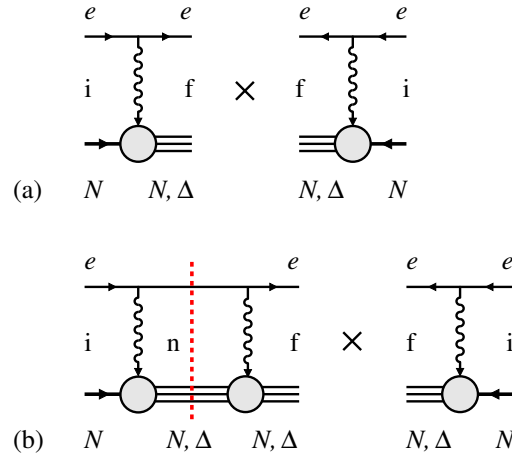
Figure 2: Inclusive electron-nucleon scattering cross section with N and \Delta final states in large- N_c limit. (a) Spin-independent cross section from square of e^2 amplitudes. The circle denotes the electromagnetic current matrix element between baryon states. (b) Spin-dependent cross section from interference of e^4 and e^2 amplitudes.
