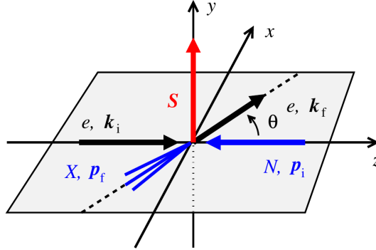
Figure 1: Inclusive electron-nucleon scattering in the electron-nucleon CM frame. The nucleon is polarized in the direction normal to the scattering plane.
