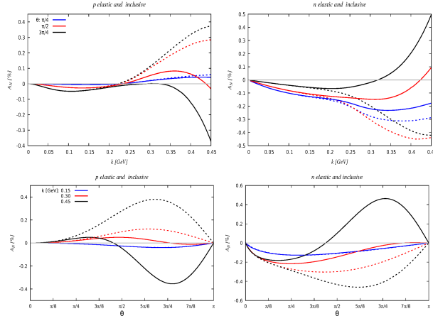
Figure 4: A_N vs k (top) and A_N vs \theta (bottom) with inclusion of form factors and \Delta width. Elastic (dashed) and inclusive (solid).
