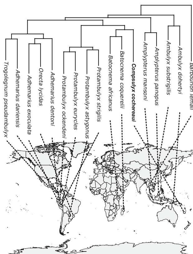
Fig. 3. The Bayesian topology plotted onto a map of the Earth.
