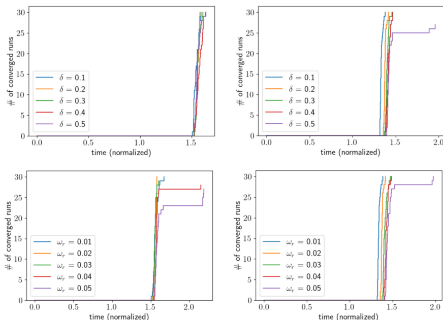
FIG. 17. Ensemble convergence of ASJ-R in the presence of malevolent corruption for the Poisson benchmark (left column) and the MGG system (right column) with recovery time \omega_r = 0.02 s and various offset magnitudes \delta (top row) and various recovery times \omega_r and offset magnitude \delta = 0.2 (bottom row). The convergence behavior is comparable for the two linear systems.
