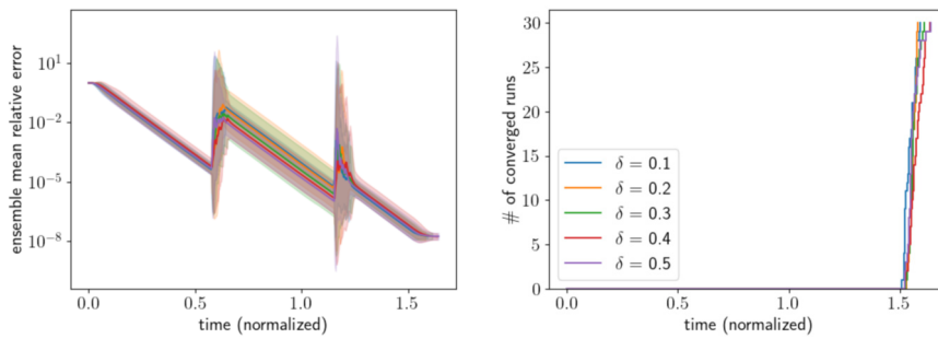
FIG. 11. Ensemble convergence of ASJ-R with malevolent corruption with time to failure \omega_f = 2 s ( t \approx 0.6 in normalized time), recovery time \omega_r = 0.02 s, and various offset magnitudes \delta . Convergence is achieved for all runs, resulting in times to solution around 1.5 times longer than without corruption.
