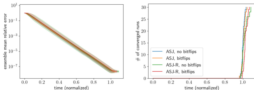
FIG. 3. Ensemble convergence of ASJ and ASJ-R with bit flip probability p = 0.01 , with double floating point flips limited to the lower mantissa \text{IE}^3([0-25]) . Convergence is achieved in all ASJ and ASJ-R runs, with times to solution comparable to the respective baseline (no corruption) values.
