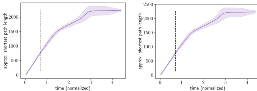
FIG. 7. Approximate shortest path length \tilde{s}_i(t) used by the ASJ-R algorithm with bit flip probability p = 0.01 , with double float point flips limited to the sign bit \text{IE}^3([26-51]) (left: i = 7 ; right: i = 9 ). The approximate shortest path length reaches 750 at around the time the stagnation period ends in Figure 6 (denoted by dashed black line).
