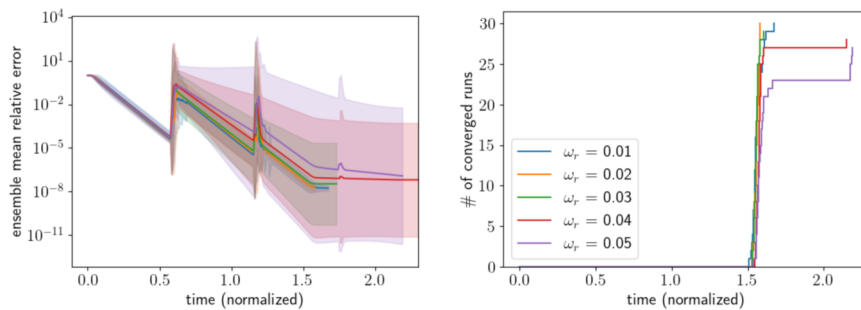
FIG. 12. Ensemble convergence of ASJ-R with malevolent corruption with time to failure \omega_f = 2 s, various recovery times \omega_r , and offset magnitude \delta = 0.2 . Convergence is achieved for all runs with \omega_r = 0.01 s and \omega_r = 0.02 and almost all runs with larger \omega_r , resulting in times to solution around 1.5 times longer than without corruption.
