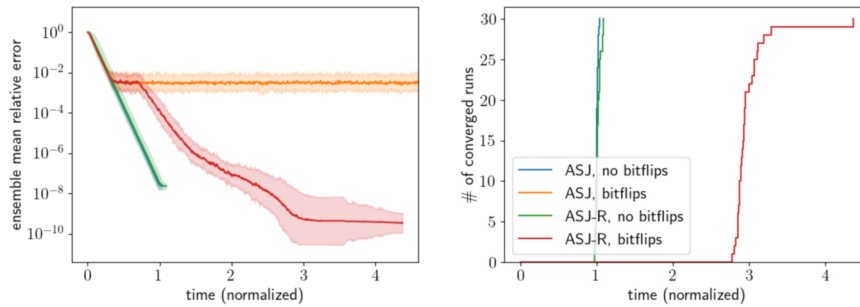
FIG. 6. Ensemble convergence of ASJ and ASJ-R with bit flip probability p = 0.01 , with double floating point flips limited to the upper mantissa \text{IE}^3([26-51]) . Convergence is lost for all of the ASJ runs and achieved for all ASJ-R runs. The times to solution of the convergent runs are longer than those of sign bit flips (Figure 4); however, the times to tolerance \epsilon = 10^{-5} are about the same as sign bit flips.
