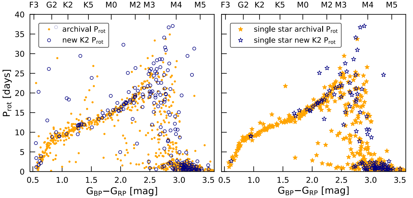
Figure 6. Gaia color–period distribution for Praesepe rotators. Rotators found prior to this work are in orange. New rotators are in navy. Left: The entire rotator sample with likely binaries included. Right: The likely single-star rotator sample.
