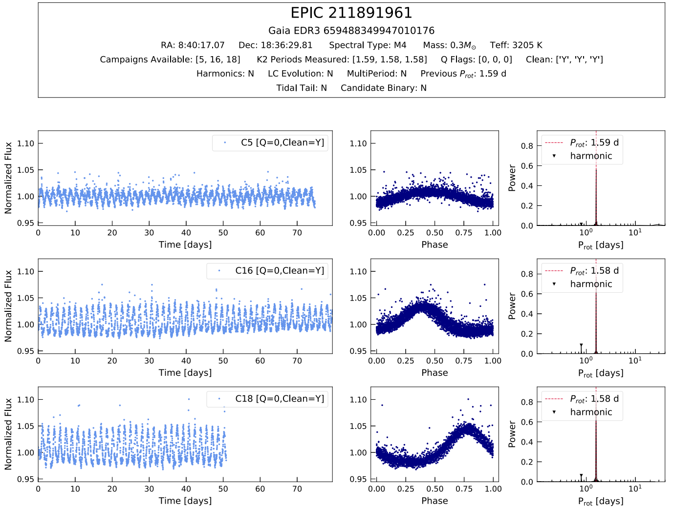
Figure 8. Example figure set for a star with multiple K2 light curves and P_{\text{rot}} measured, EPIC 211891961. Top: Information about the star including the EPIC ID, Gaia EDR3 name, R.A., decl., mass, effective temperature, campaigns observed, periods measured, quality flags assigned, clean detection flag, harmonics detected across campaigns, light-curve evolution observed, multiple periods observed, previous P_{\text{rot}} measured, tidal-tail status, and binary status. Left column: Light curves from C5, C16, and C18. Middle column: Light curves phase-folded to P_{\text{rot}} measured from each campaign. Right column: LS periodograms. The complete figure (825 images) set is available in the online journal.
