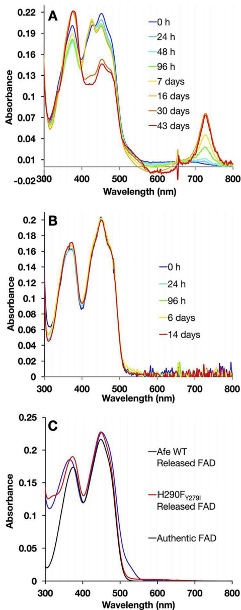
Fig. 9 8-Formyl flavin formation at pH 9 in WT- vs. H290FY279I-ETF. Visible spectra of (A) WT-ETF and (B) H290FY279I-ETF at pH 9 were recorded at intervals over a period of 144 h. Visible spectra of the WT demonstrated an increase in absorbance at 424 nm characteristic of 8fF and the presence of NSQ which decreased over time while bands near 530 and 730 nm increased. Meanwhile, the H290FY279I variant remained unmodified and fully oxidized at pH 9. The spectra collected over 384 h for WT were normalized using the isosbestic point at 406 nm and the spectra collected after 30 days and 43 days resembled 8fF ASQ and were normalized using 660 nm. (C) Comparison flavins released from WT- and H290FY279I-ETF after full reaction at pH 9. Flavin released from WT-ETF deviated from authentic FAD in a blue-shifted band II and a prominent shoulder near 530 nm.
