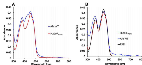
Fig. 4 Spectral signatures of flavin modification are absent from H290FY279I. (A) Spectra of the WT (blue) and H290FY279I (red) ETF; (B) spectra of flavins released from the WT (blue) and H290FY279I (red). Visible spectra of 20 \mu M WT and variant H290FY279I in 50 mM PO 4 buffer pH 7 and their released flavins along with free FAD were recorded. In A, the ETF spectra of the WT and H290FY279I are distinguished by the absence from the latter of the features near 415 nm attributed to 8-formyl flavin (8fF). In (B) the spectrum of the flavin released from the WT deviates from the authentic FAD in having a stronger and blue-shifted band II, near 370 nm, whereas flavin from the variant resembles authentic FAD. Equally strong band I and a blue shifted band II are characteristic of 8fF. Since Afe ETF contains two FADs, the signals of both contribute to all spectra, and changes affecting the ET-FAD are proportionately less significant due to admixture of the unchanged spectrum of Bf-FAD.
