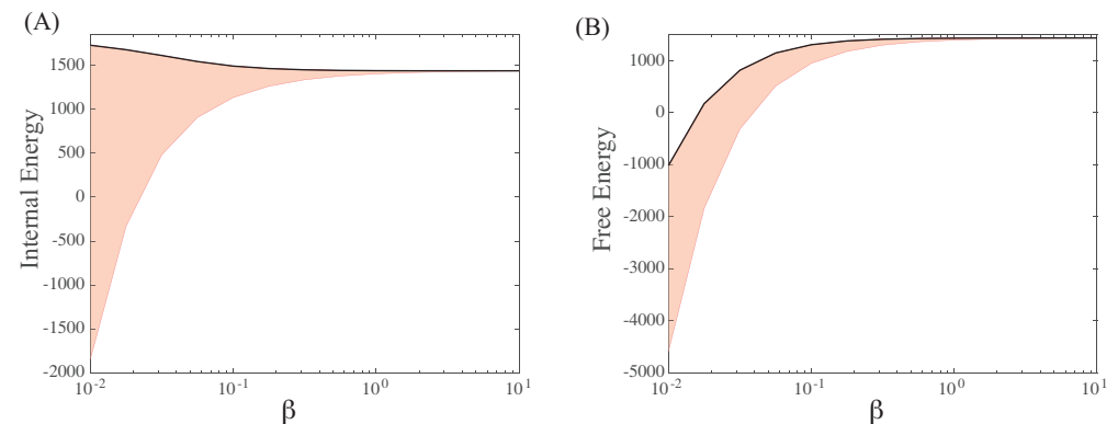
Figure 1. Convergence of the internal energy U_{\beta}^{MF} (A) and free energy F_{\beta}^{MF} (B) as a function of \beta when solving the multi-task assignment problem with the cost matrix C_1 , such that each agent can perform up to 4 tasks, may be idle, and all 8 tasks are performed. On both panels, we show the bounds on the expected value for the optimal cost U^* as shaded areas (see text for details).
