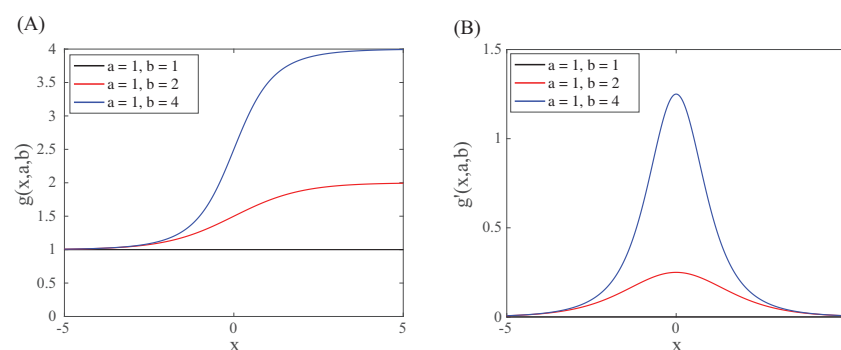
Figure A1. Examples of g(x, a, b) (A) and its derivative g'(x, a, b) (B) for a = 1, b = 1 (black), a = 1, b = 2 , (red), and a = 1, b = 4 (blue).
